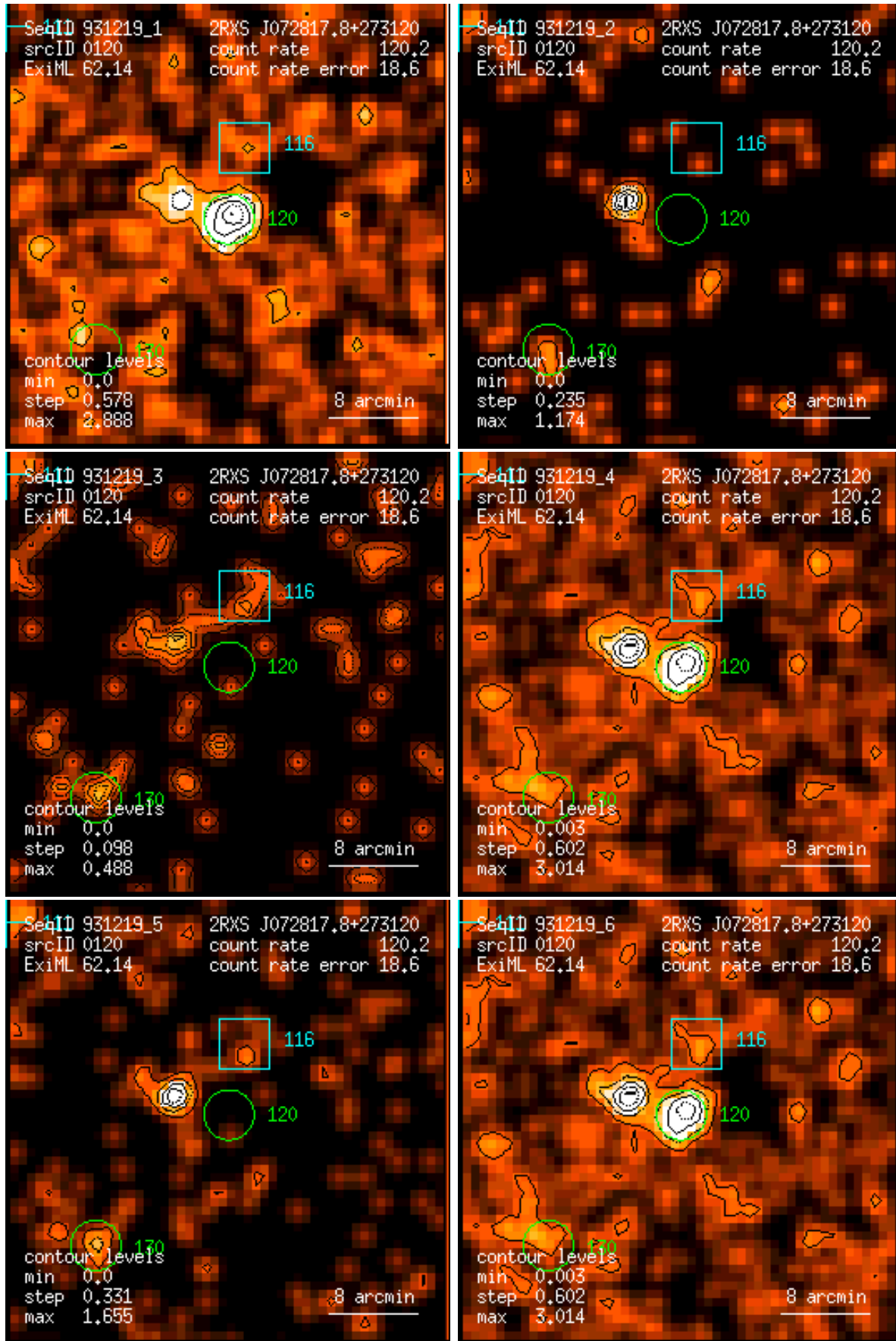
Figure 120: RASS 931219: detection 0120: band rate images, Gaussian filter: (1) PSPC channels 11 – 41, (2) 52 – 90, (3) 91 – 201, (4) 11 – 235, (5) 52 – 201, (6) 11 – 201. Broad band rates in counts/ks. Band rate contour levels in counts/ks/arcmin 2 .
