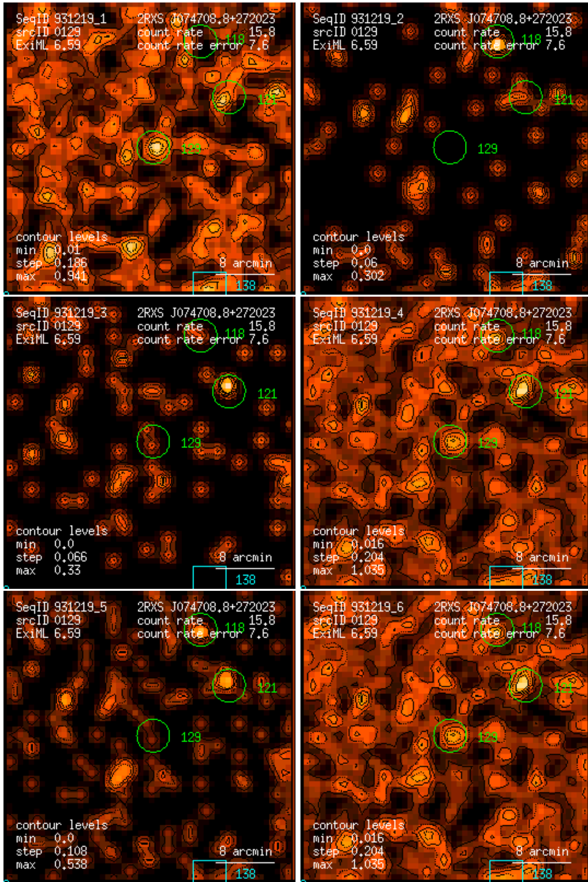
Figure 129: RASS 931219: detection 0129: band rate images, Gaussian filter: (1) PSPC channels 11 – 41, (2) 52 – 90, (3) 91 – 201, (4) 11 – 235, (5) 52 – 201, (6) 11 – 201. Broad band rates in counts/ks. Band rate contour levels in counts/ks/arcmin 2 .
