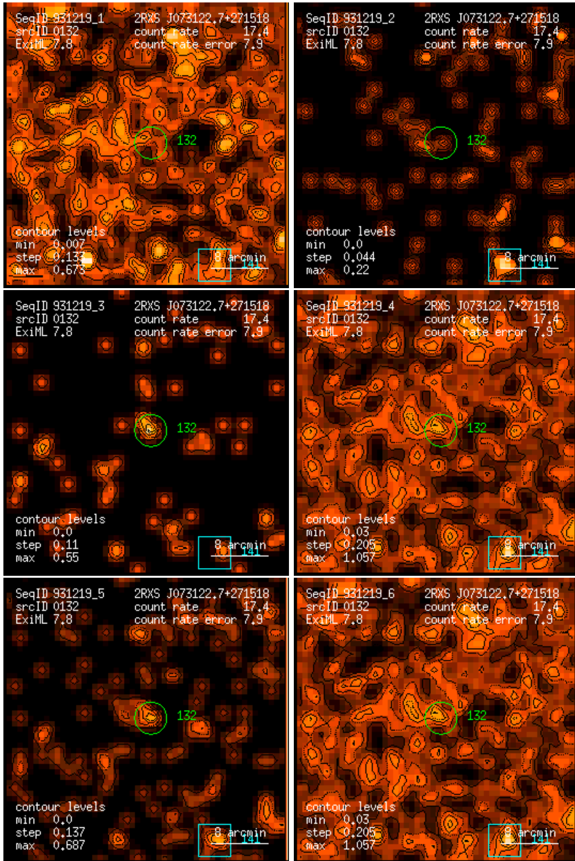
Figure 132: RASS 931219: detection 0132: band rate images, Gaussian filter: (1) PSPC channels 11 – 41, (2) 52 – 90, (3) 91 – 201, (4) 11 – 235, (5) 52 – 201, (6) 11 – 201. Broad band rates in counts/ks. Band rate contour levels in counts/ks/arcmin 2 .
