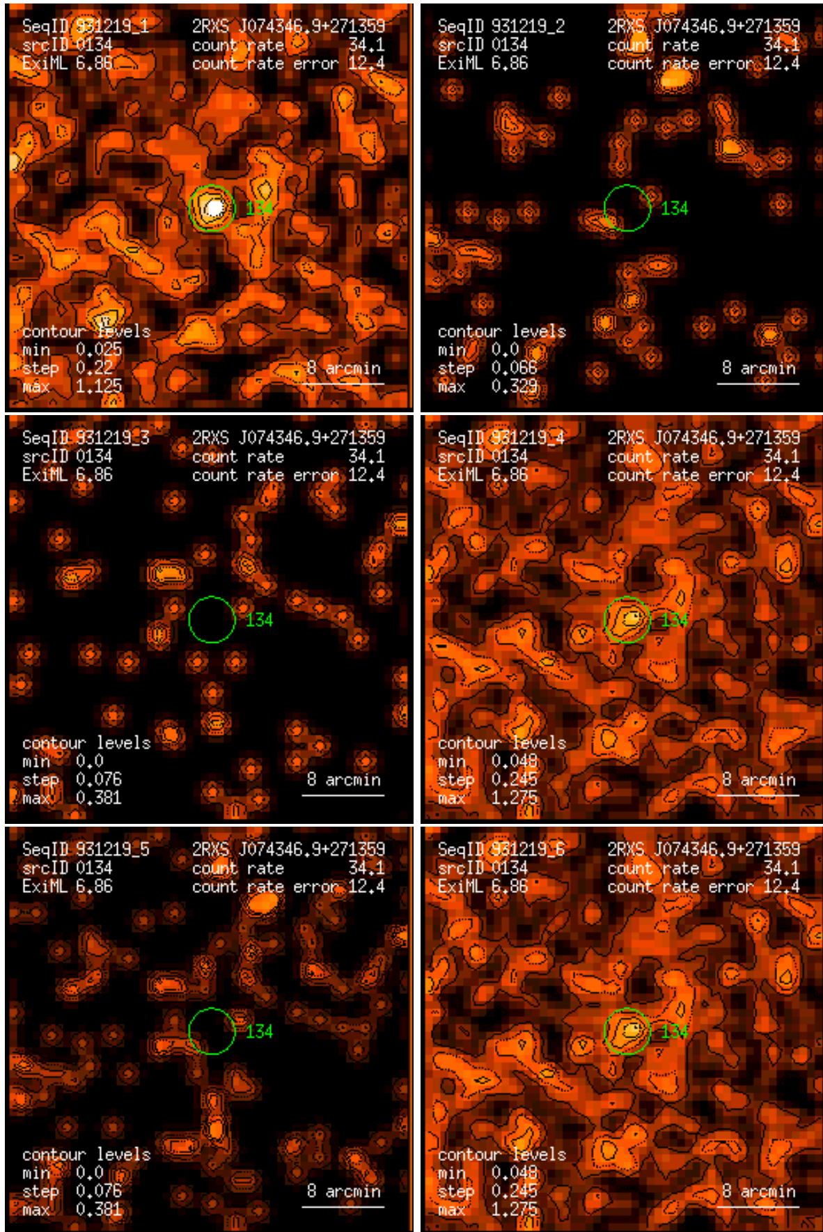
Figure 134: RASS 931219: detection 0134: band rate images, Gaussian filter: (1) PSPC channels 11 – 41, (2) 52 – 90, (3) 91 – 201, (4) 11 – 235, (5) 52 – 201, (6) 11 – 201. Broad band rates in counts/ks. Band rate contour levels in counts/ks/arcmin 2 .
