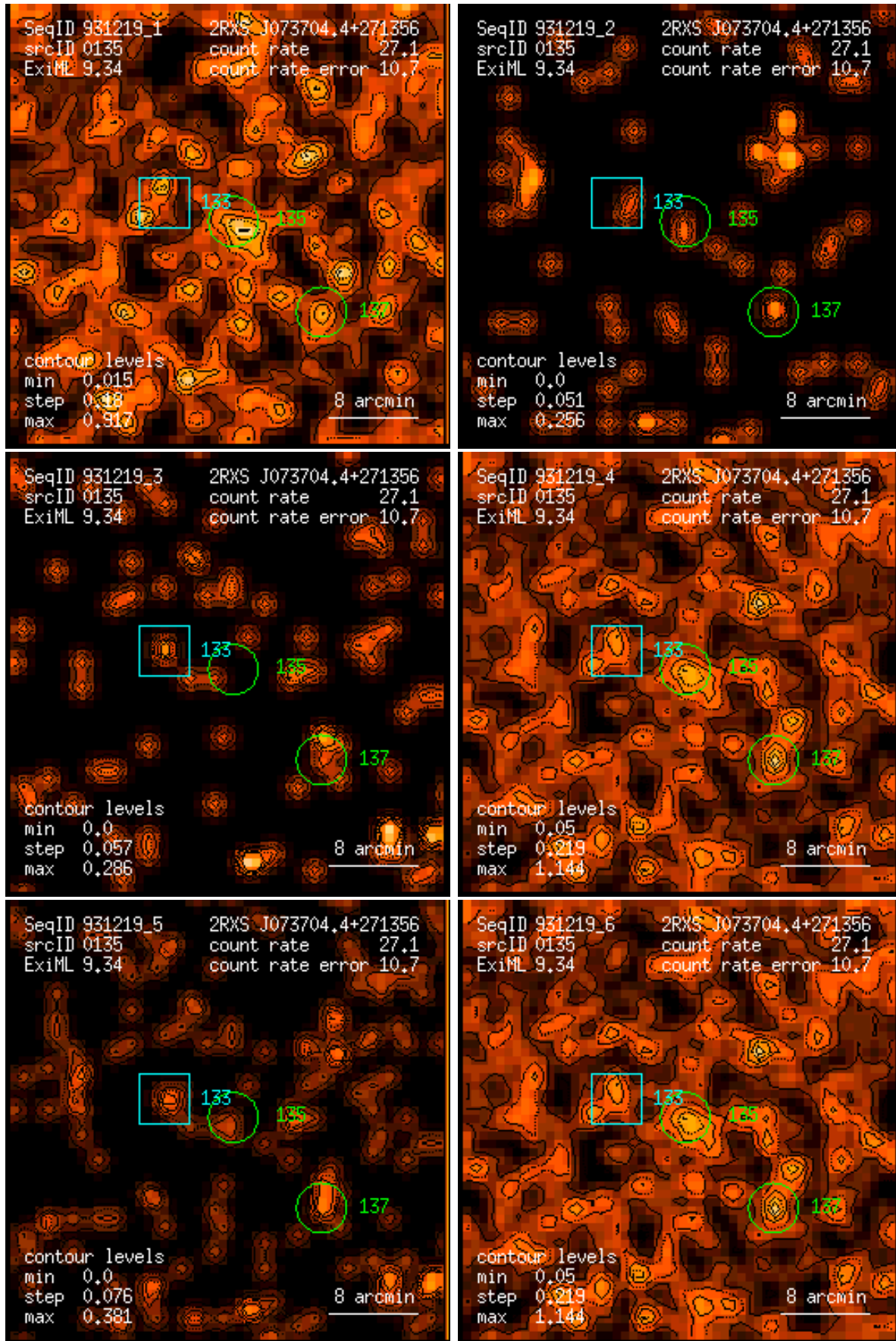
Figure 135: RASS 931219: detection 0135: band rate images, Gaussian filter: (1) PSPC channels 11 – 41, (2) 52 – 90, (3) 91 – 201, (4) 11 – 235, (5) 52 – 201, (6) 11 – 201. Broad band rates in counts/ks. Band rate contour levels in counts/ks/arcmin 2 .
