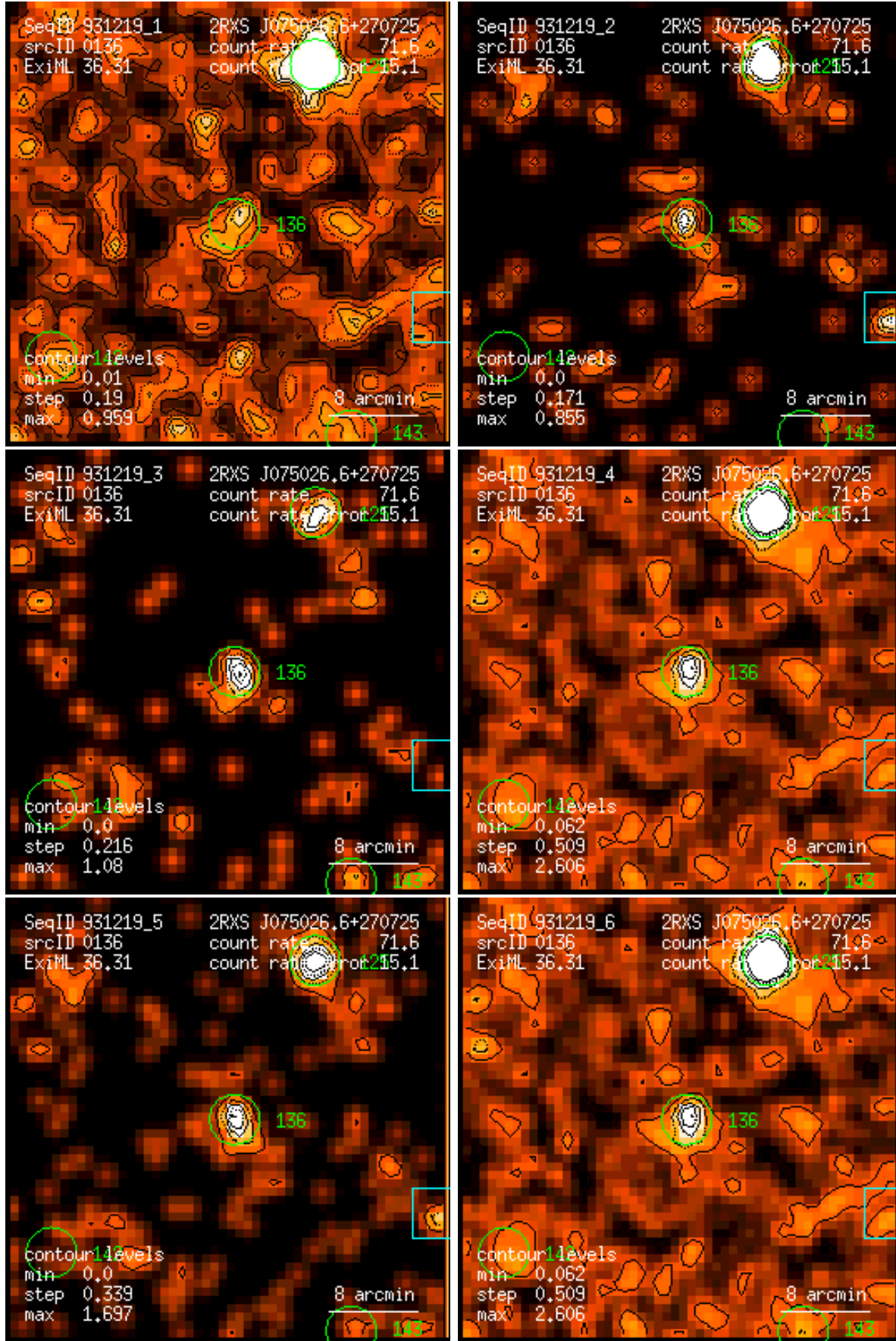
Figure 136: RASS 931219: detection 0136: band rate images, Gaussian filter: (1) PSPC channels 11 – 41, (2) 52 – 90, (3) 91 – 201, (4) 11 – 235, (5) 52 – 201, (6) 11 – 201. Broad band rates in counts/ks. Band rate contour levels in counts/ks/arcmin 2 .
