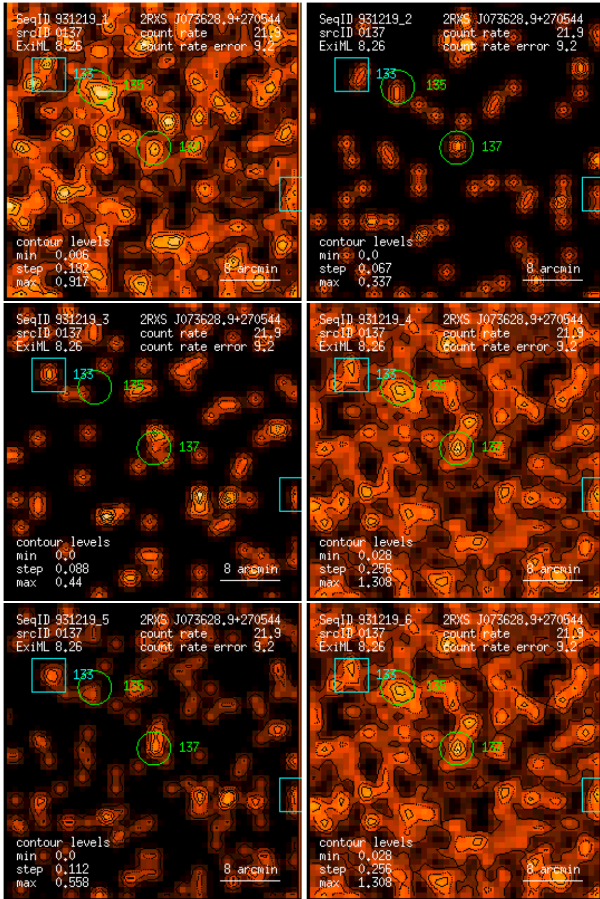
Figure 137: RASS 931219: detection 0137: band rate images, Gaussian filter: (1) PSPC channels 11 – 41, (2) 52 – 90, (3) 91 – 201, (4) 11 – 235, (5) 52 – 201, (6) 11 – 201. Broad band rates in counts/ks. Band rate contour levels in counts/ks/arcmin 2 .
