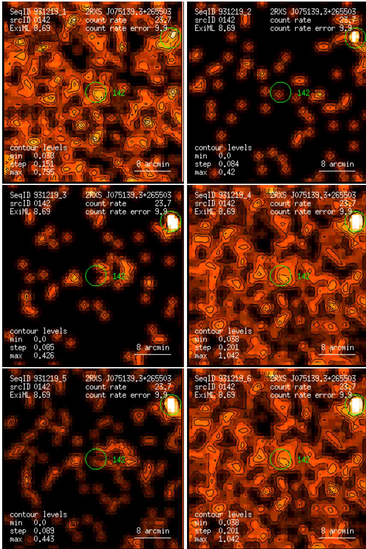
Figure 142: RASS 931219: detection 0142: band rate images, Gaussian filter: (1) PSPC channels 11 – 41, (2) 52 – 90, (3) 91 – 201, (4) 11 – 235, (5) 52 – 201, (6) 11 – 201. Broad band rates in counts/ks. Band rate contour levels in counts/ks/arcmin 2 .
