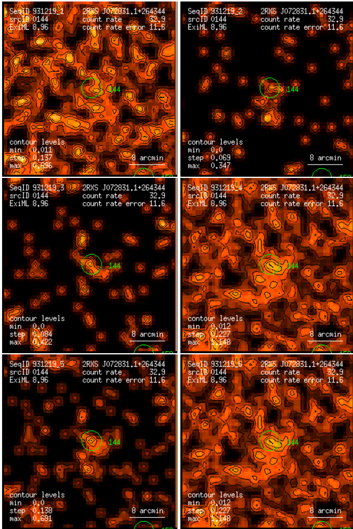
Figure 144: RASS 931219: detection 0144: band rate images, Gaussian filter: (1) PSPC channels 11 – 41, (2) 52 – 90, (3) 91 – 201, (4) 11 – 235, (5) 52 – 201, (6) 11 – 201. Broad band rates in counts/ks. Band rate contour levels in counts/ks/arcmin 2 .
