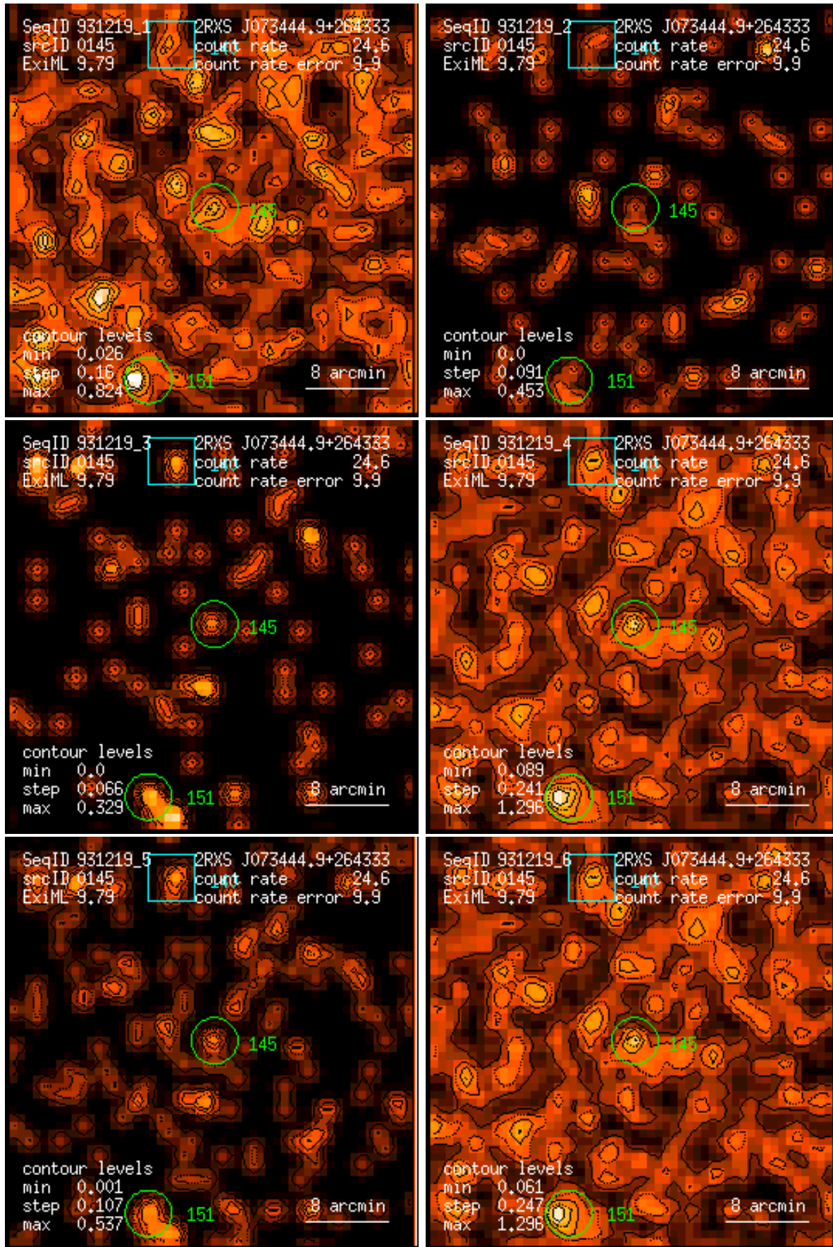
Figure 145: RASS 931219: detection 0145: band rate images, Gaussian filter: (1) PSPC channels 11 – 41, (2) 52 – 90, (3) 91 – 201, (4) 11 – 235, (5) 52 – 201, (6) 11 – 201. Broad band rates in counts/ks. Band rate contour levels in counts/ks/arcmin 2 .
