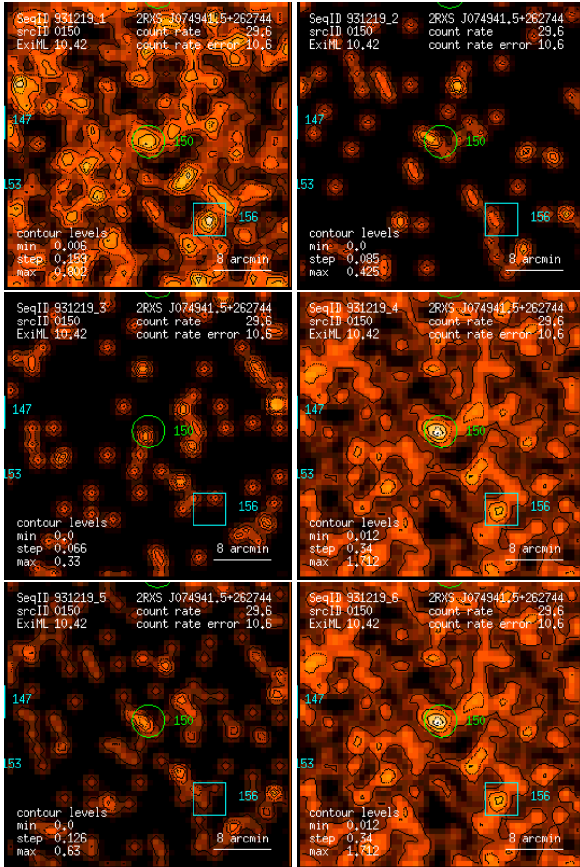
Figure 150: RASS 931219: detection 0150: band rate images, Gaussian filter: (1) PSPC channels 11 – 41, (2) 52 – 90, (3) 91 – 201, (4) 11 – 235, (5) 52 – 201, (6) 11 – 201. Broad band rates in counts/ks. Band rate contour levels in counts/ks/arcmin 2 .
