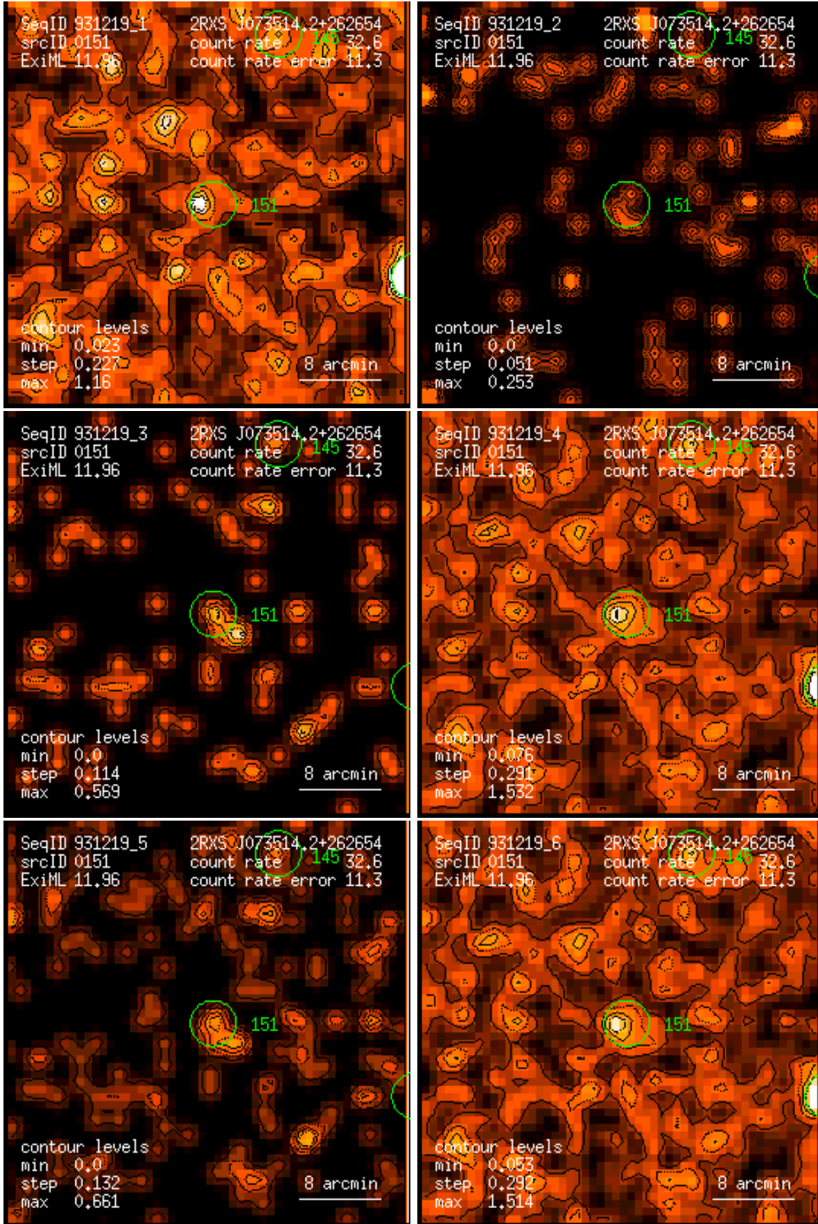
Figure 151: RASS 931219: detection 0151: band rate images, Gaussian filter: (1) PSPC channels 11 – 41, (2) 52 – 90, (3) 91 – 201, (4) 11 – 235, (5) 52 – 201, (6) 11 – 201. Broad band rates in counts/ks. Band rate contour levels in counts/ks/arcmin 2 .
