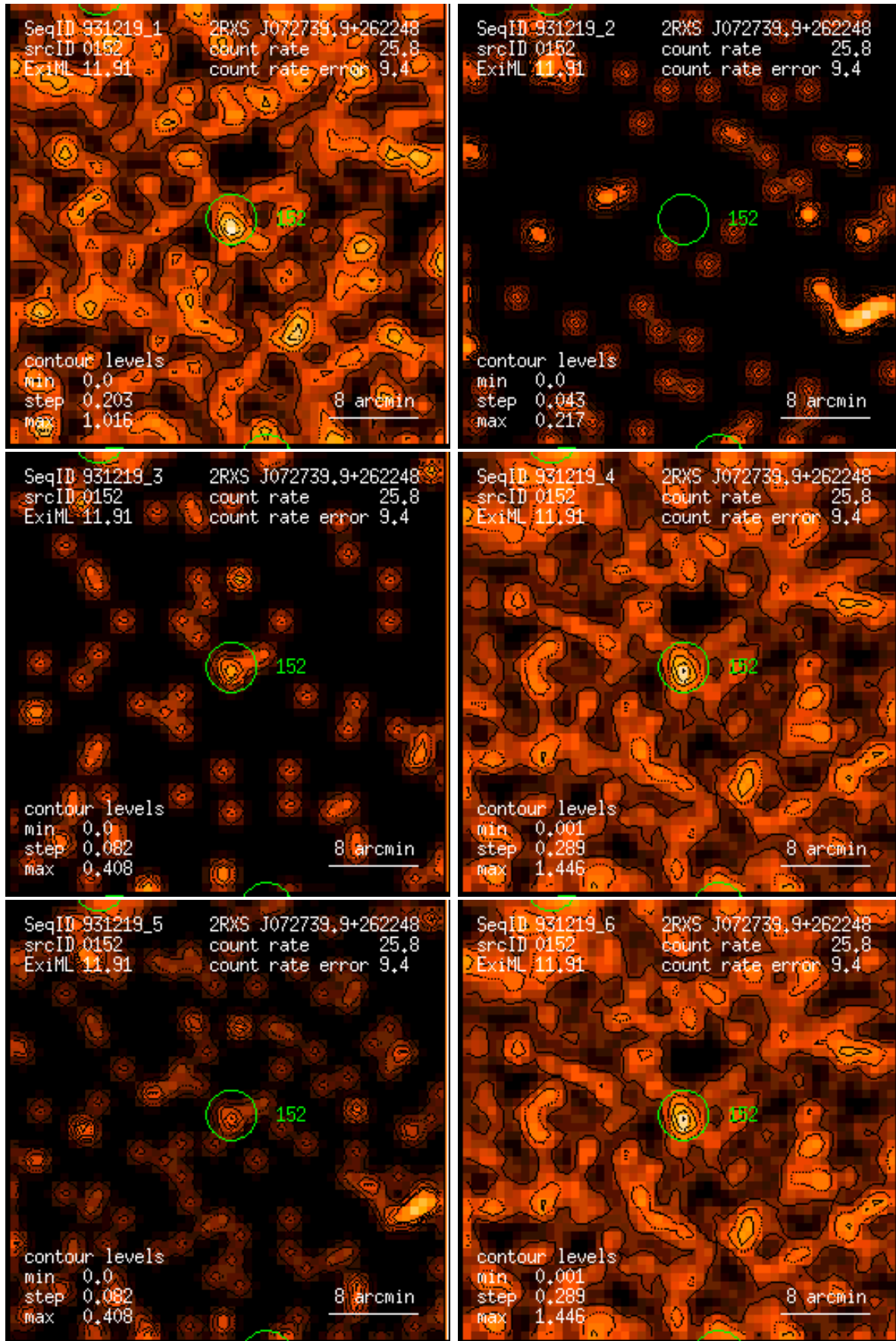
Figure 152: RASS 931219: detection 0152: band rate images, Gaussian filter: (1) PSPC channels 11 – 41, (2) 52 – 90, (3) 91 – 201, (4) 11 – 235, (5) 52 – 201, (6) 11 – 201. Broad band rates in counts/ks. Band rate contour levels in counts/ks/arcmin 2 .
