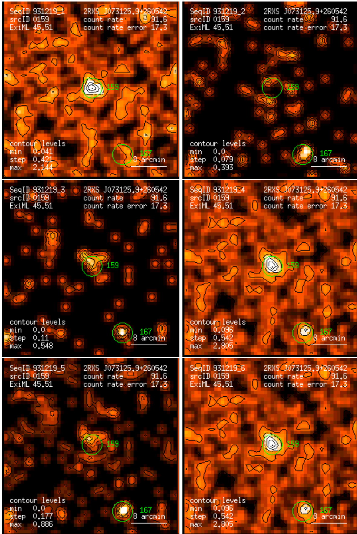
Figure 159: RASS 931219: detection 0159: band rate images, Gaussian filter: (1) PSPC channels 11 – 41, (2) 52 – 90, (3) 91 – 201, (4) 11 – 235, (5) 52 – 201, (6) 11 – 201. Broad band rates in counts/ks. Band rate contour levels in counts/ks/arcmin 2 .
