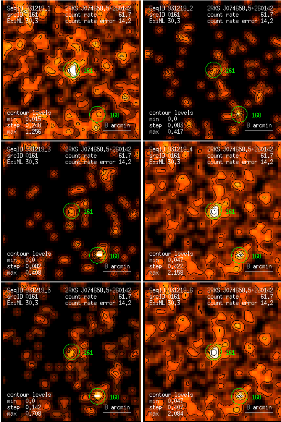
Figure 161: RASS 931219: detection 0161: band rate images, Gaussian filter: (1) PSPC channels 11 – 41, (2) 52 – 90, (3) 91 – 201, (4) 11 – 235, (5) 52 – 201, (6) 11 – 201. Broad band rates in counts/ks. Band rate contour levels in counts/ks/arcmin 2 .
