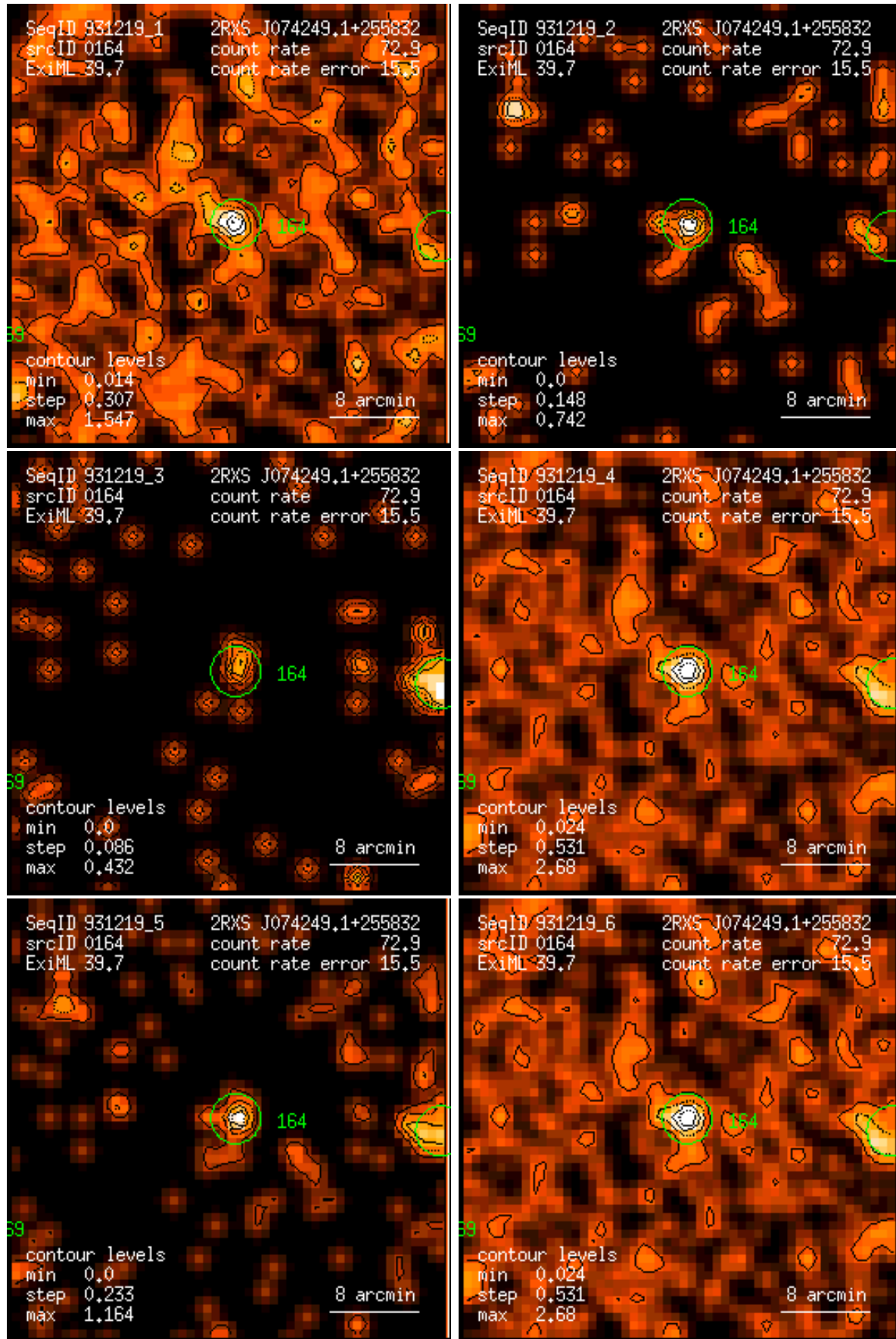
Figure 164: RASS 931219: detection 0164: band rate images, Gaussian filter: (1) PSPC channels 11 – 41, (2) 52 – 90, (3) 91 – 201, (4) 11 – 235, (5) 52 – 201, (6) 11 – 201. Broad band rates in counts/ks. Band rate contour levels in counts/ks/arcmin 2 .
