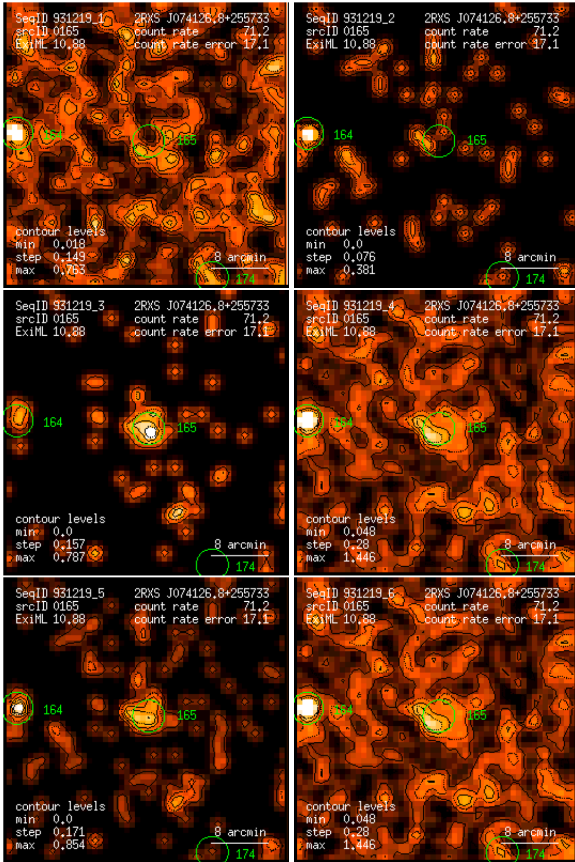
Figure 165: RASS 931219: detection 0165: band rate images, Gaussian filter: (1) PSPC channels 11 – 41, (2) 52 – 90, (3) 91 – 201, (4) 11 – 235, (5) 52 – 201, (6) 11 – 201. Broad band rates in counts/ks. Band rate contour levels in counts/ks/arcmin 2 .
