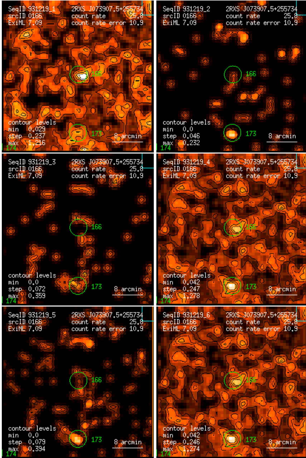
Figure 166: RASS 931219: detection 0166: band rate images, Gaussian filter: (1) PSPC channels 11 – 41, (2) 52 – 90, (3) 91 – 201, (4) 11 – 235, (5) 52 – 201, (6) 11 – 201. Broad band rates in counts/ks. Band rate contour levels in counts/ks/arcmin 2 .
