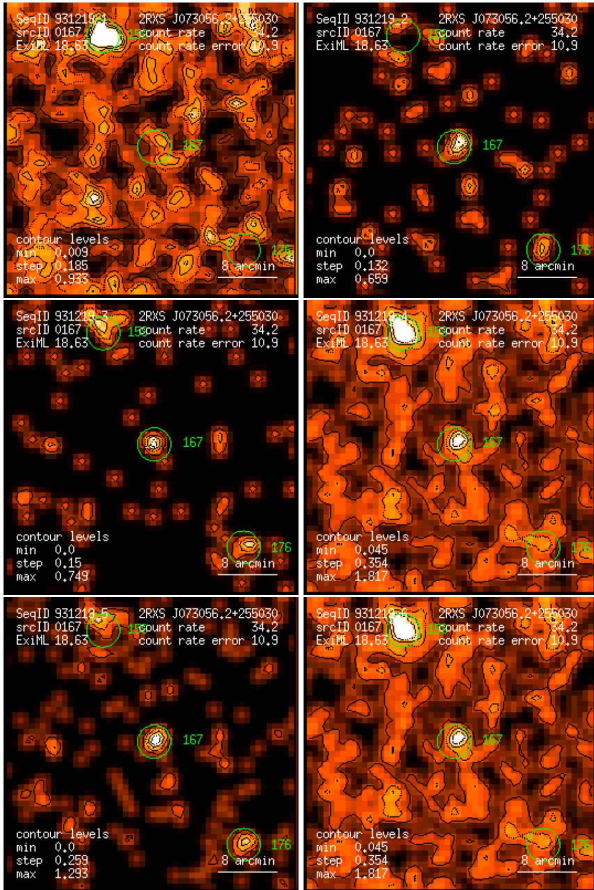
Figure 167: RASS 931219: detection 0167: band rate images, Gaussian filter: (1) PSPC channels 11 – 41, (2) 52 – 90, (3) 91 – 201, (4) 11 – 235, (5) 52 – 201, (6) 11 – 201. Broad band rates in counts/ks. Band rate contour levels in counts/ks/arcmin 2 .
