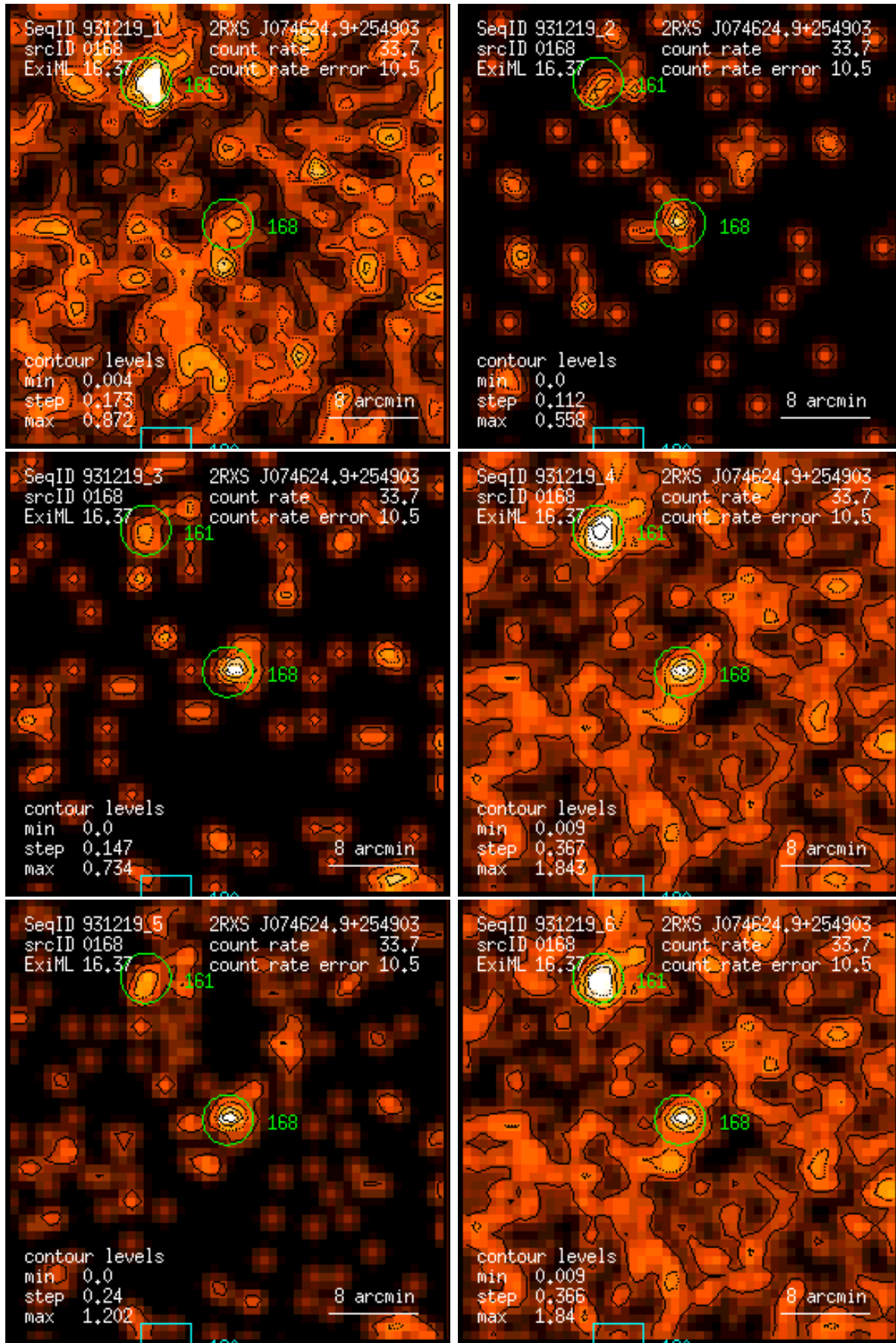
Figure 168: RASS 931219: detection 0168: band rate images, Gaussian filter: (1) PSPC channels 11 – 41, (2) 52 – 90, (3) 91 – 201, (4) 11 – 235, (5) 52 – 201, (6) 11 – 201. Broad band rates in counts/ks. Band rate contour levels in counts/ks/arcmin 2 .
