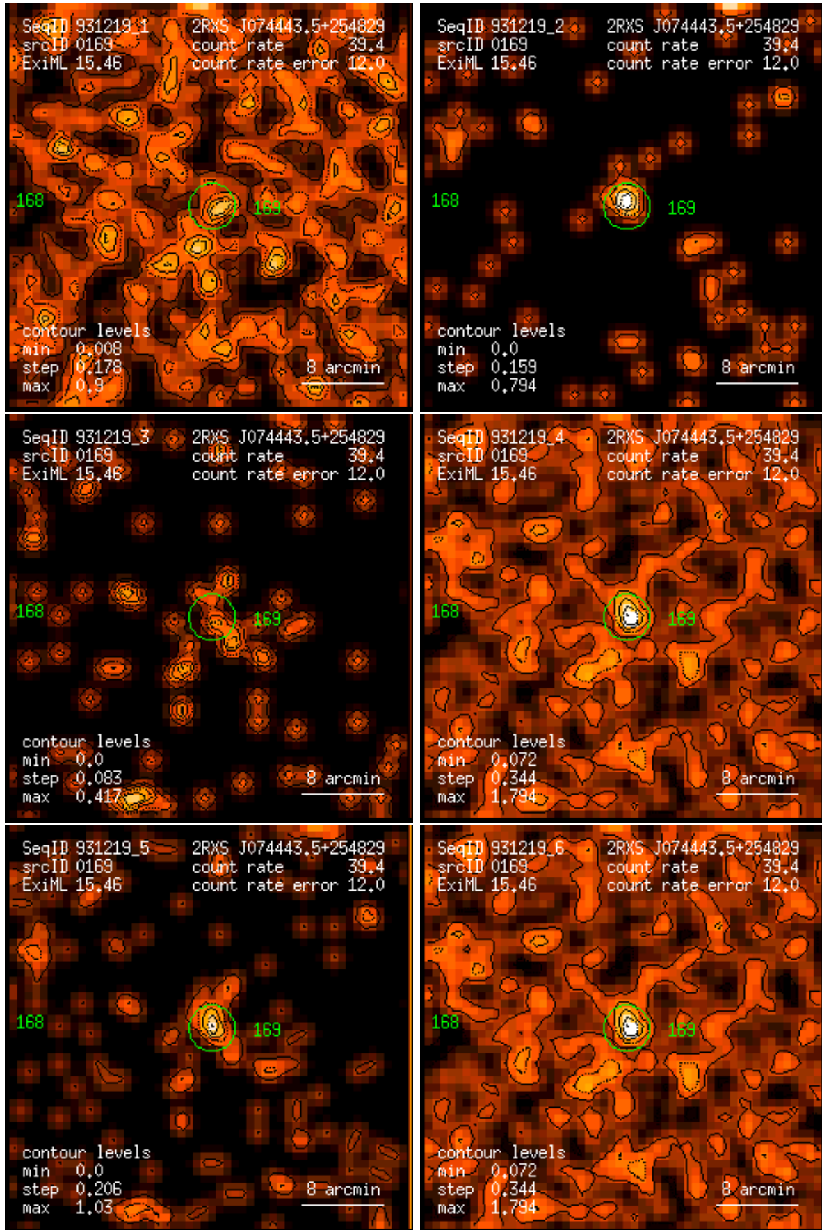
Figure 169: RASS 931219: detection 0169: band rate images, Gaussian filter: (1) PSPC channels 11 – 41, (2) 52 – 90, (3) 91 – 201, (4) 11 – 235, (5) 52 – 201, (6) 11 – 201. Broad band rates in counts/ks. Band rate contour levels in counts/ks/arcmin 2 .
