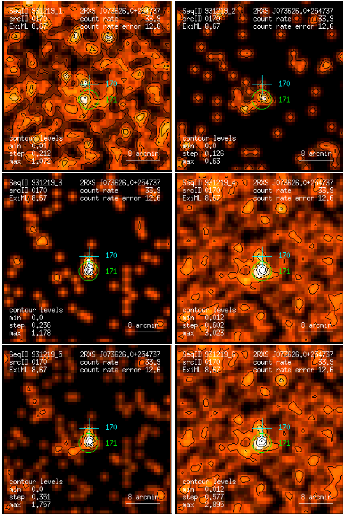
Figure 170: RASS 931219: detection 0170: band rate images, Gaussian filter: (1) PSPC channels 11 – 41, (2) 52 – 90, (3) 91 – 201, (4) 11 – 235, (5) 52 – 201, (6) 11 – 201. Broad band rates in counts/ks. Band rate contour levels in counts/ks/arcmin 2 .
