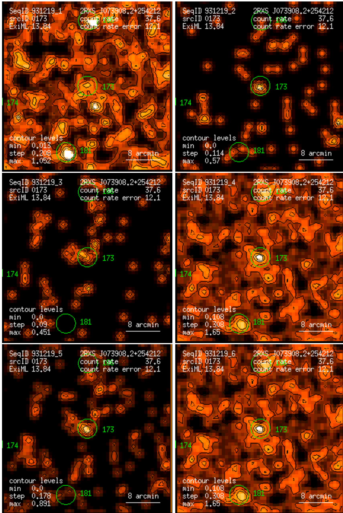
Figure 173: RASS 931219: detection 0173: band rate images, Gaussian filter: (1) PSPC channels 11 – 41, (2) 52 – 90, (3) 91 – 201, (4) 11 – 235, (5) 52 – 201, (6) 11 – 201. Broad band rates in counts/ks. Band rate contour levels in counts/ks/arcmin 2 .
