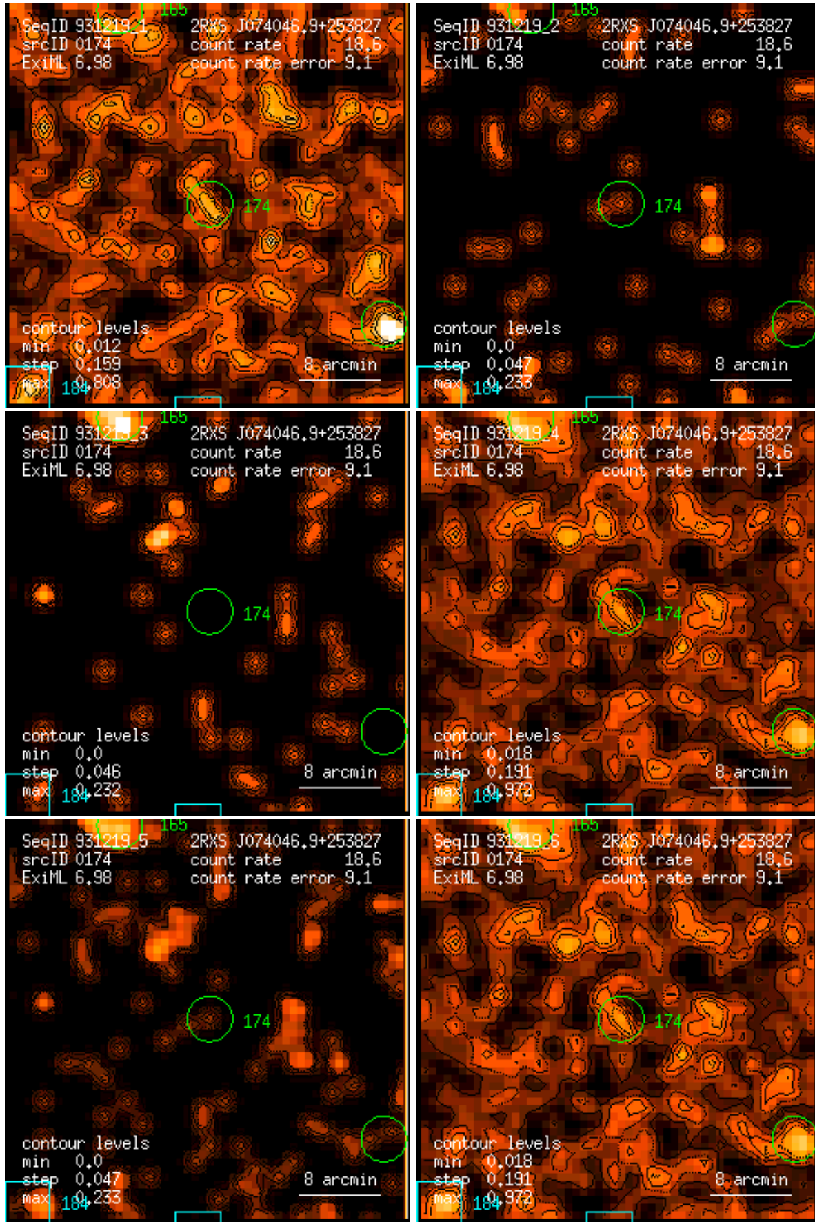
Figure 174: RASS 931219: detection 0174: band rate images, Gaussian filter: (1) PSPC channels 11 – 41, (2) 52 – 90, (3) 91 – 201, (4) 11 – 235, (5) 52 – 201, (6) 11 – 201. Broad band rates in counts/ks. Band rate contour levels in counts/ks/arcmin 2 .
