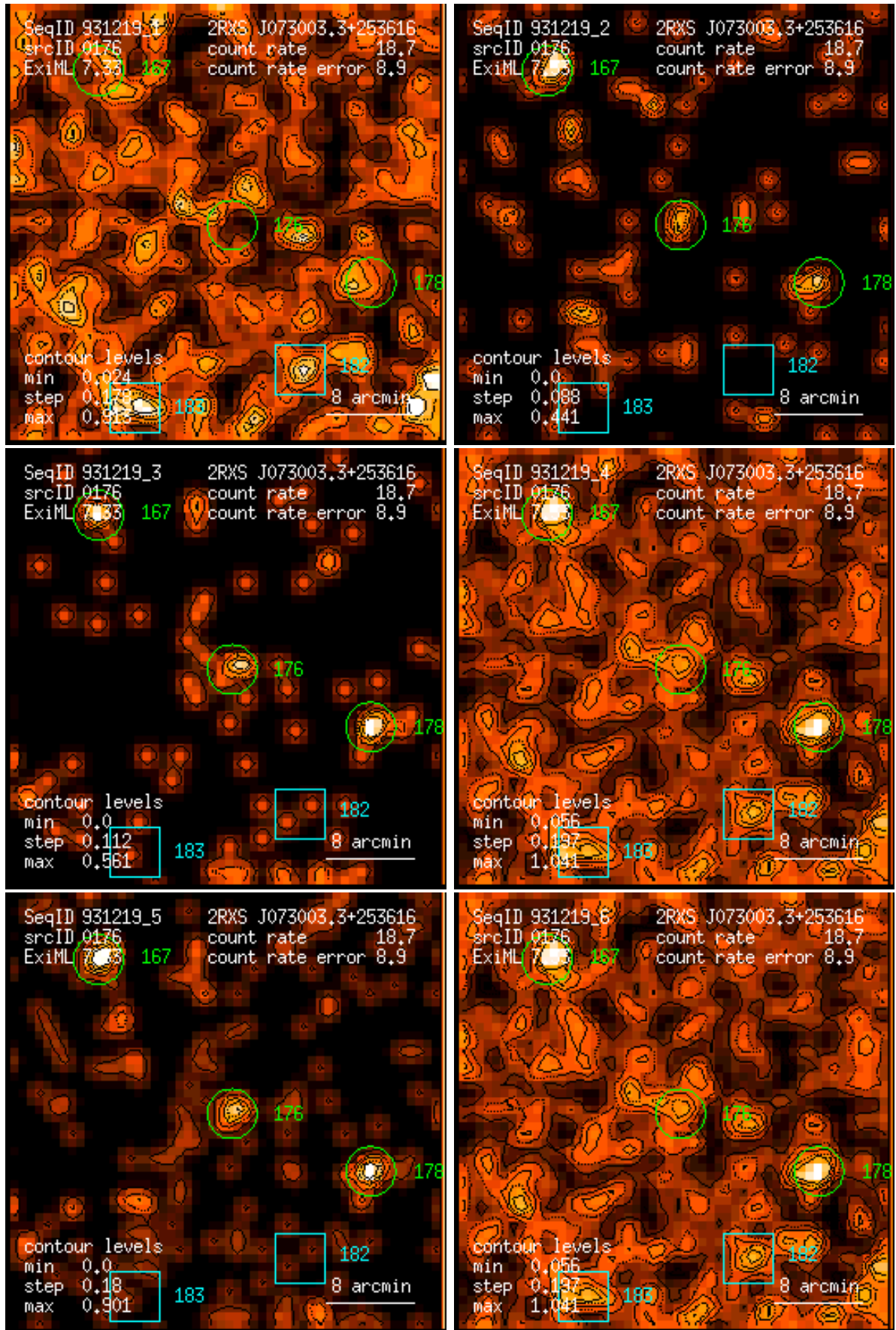
Figure 176: RASS 931219: detection 0176: band rate images, Gaussian filter: (1) PSPC channels 11 – 41, (2) 52 – 90, (3) 91 – 201, (4) 11 – 235, (5) 52 – 201, (6) 11 – 201. Broad band rates in counts/ks. Band rate contour levels in counts/ks/arcmin 2 .
