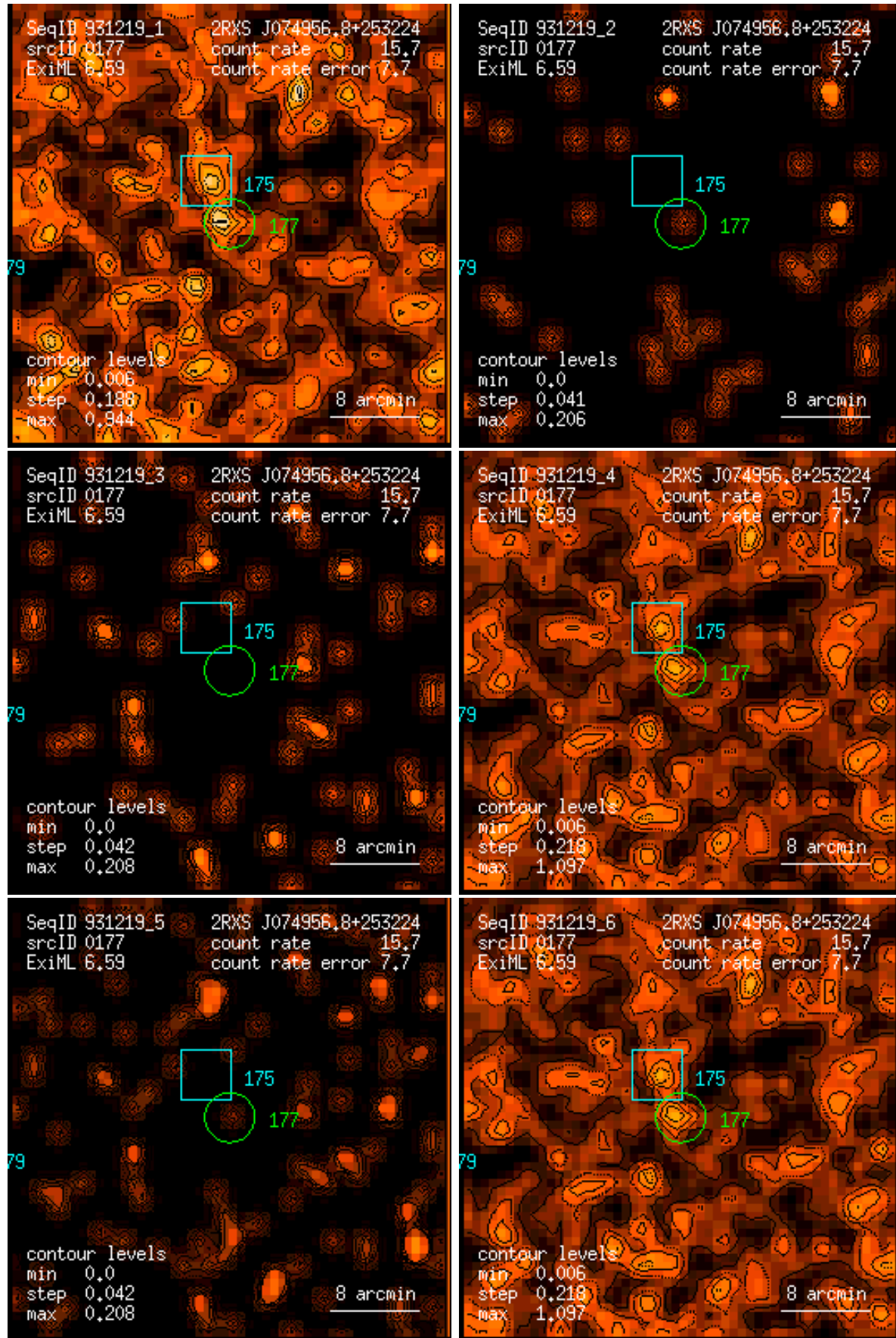
Figure 177: RASS 931219: detection 0177: band rate images, Gaussian filter: (1) PSPC channels 11 – 41, (2) 52 – 90, (3) 91 – 201, (4) 11 – 235, (5) 52 – 201, (6) 11 – 201. Broad band rates in counts/ks. Band rate contour levels in counts/ks/arcmin 2 .
