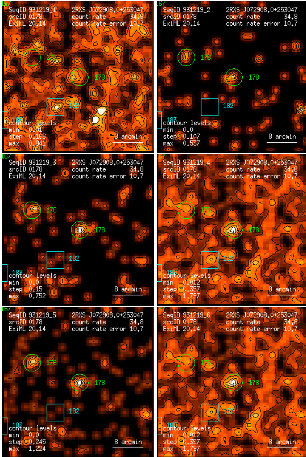
Figure 178: RASS 931219: detection 0178: band rate images, Gaussian filter: (1) PSPC channels 11 – 41, (2) 52 – 90, (3) 91 – 201, (4) 11 – 235, (5) 52 – 201, (6) 11 – 201. Broad band rates in counts/ks. Band rate contour levels in counts/ks/arcmin 2 .
