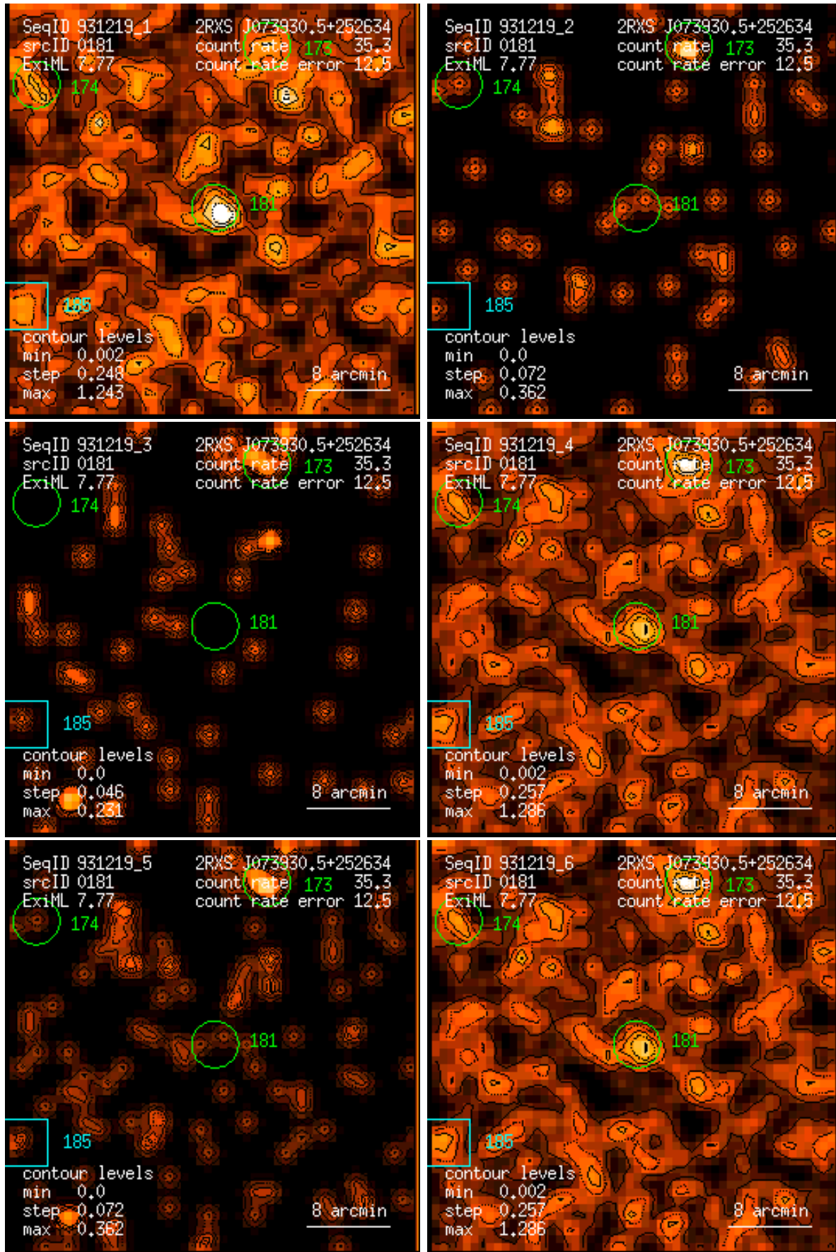
Figure 181: RASS 931219: detection 0181: band rate images, Gaussian filter: (1) PSPC channels 11 – 41, (2) 52 – 90, (3) 91 – 201, (4) 11 – 235, (5) 52 – 201, (6) 11 – 201. Broad band rates in counts/ks. Band rate contour levels in counts/ks/arcmin 2 .
