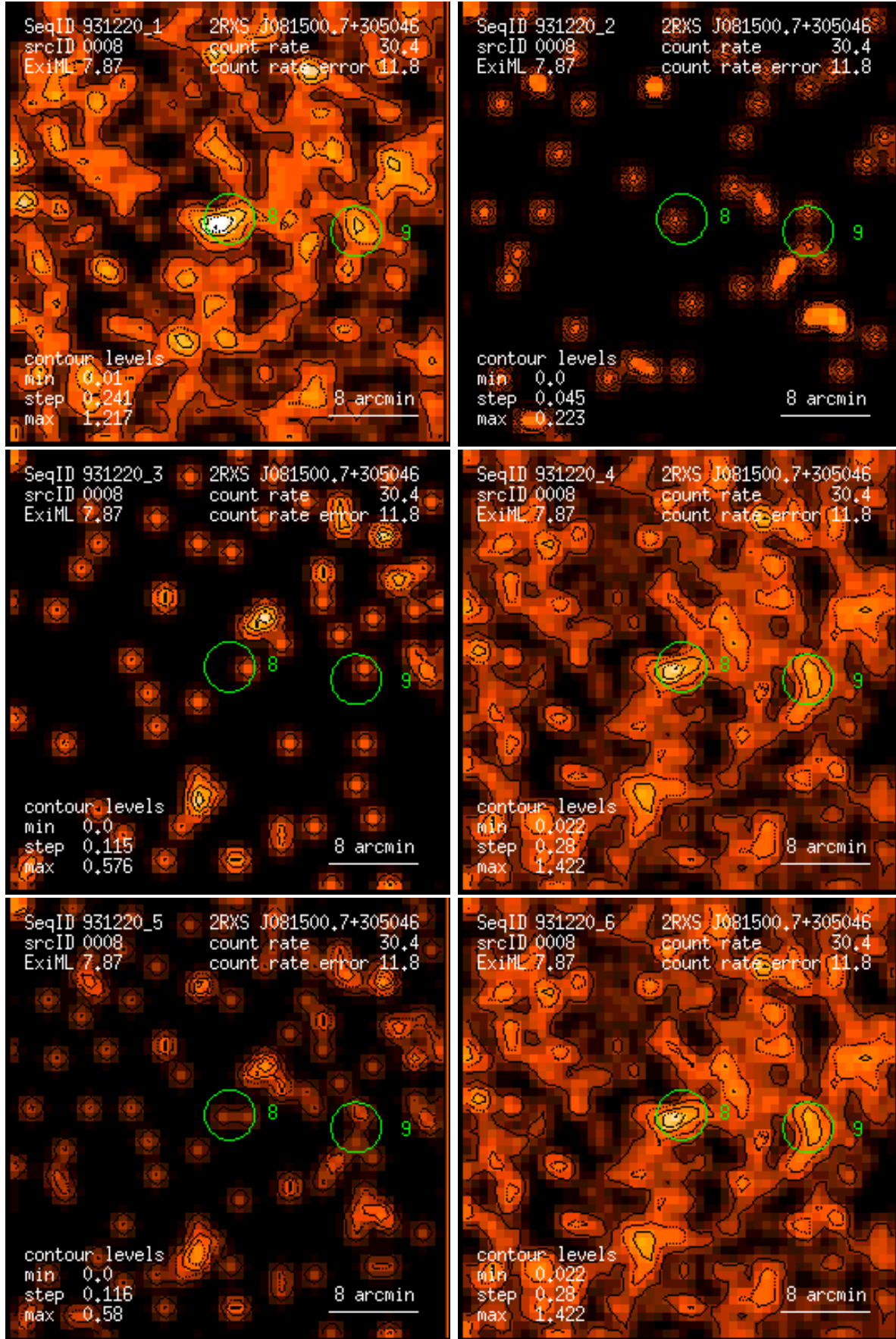
Figure 8: RASS 931220: detection 0008: band rate images, Gaussian filter: (1) PSPC channels 11 – 41, (2) 52 – 90, (3) 91 – 201, (4) 11 – 235, (5) 52 – 201, (6) 11 – 201. Broad band rates in counts/ks. Band rate contour levels in counts/ks/arcmin 2 .
