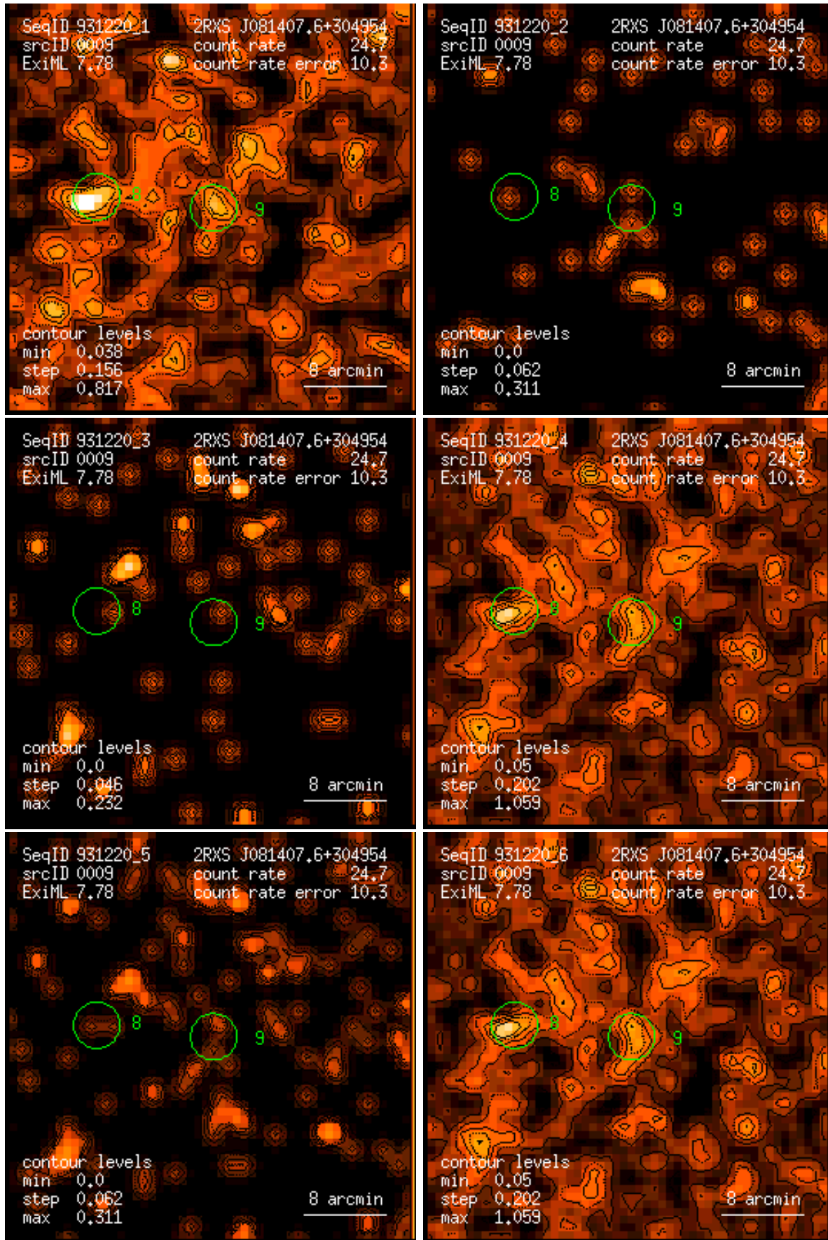
Figure 9: RASS 931220: detection 0009: band rate images, Gaussian filter: (1) PSPC channels 11 – 41, (2) 52 – 90, (3) 91 – 201, (4) 11 – 235, (5) 52 – 201, (6) 11 – 201. Broad band rates in counts/ks. Band rate contour levels in counts/ks/arcmin 2 .
