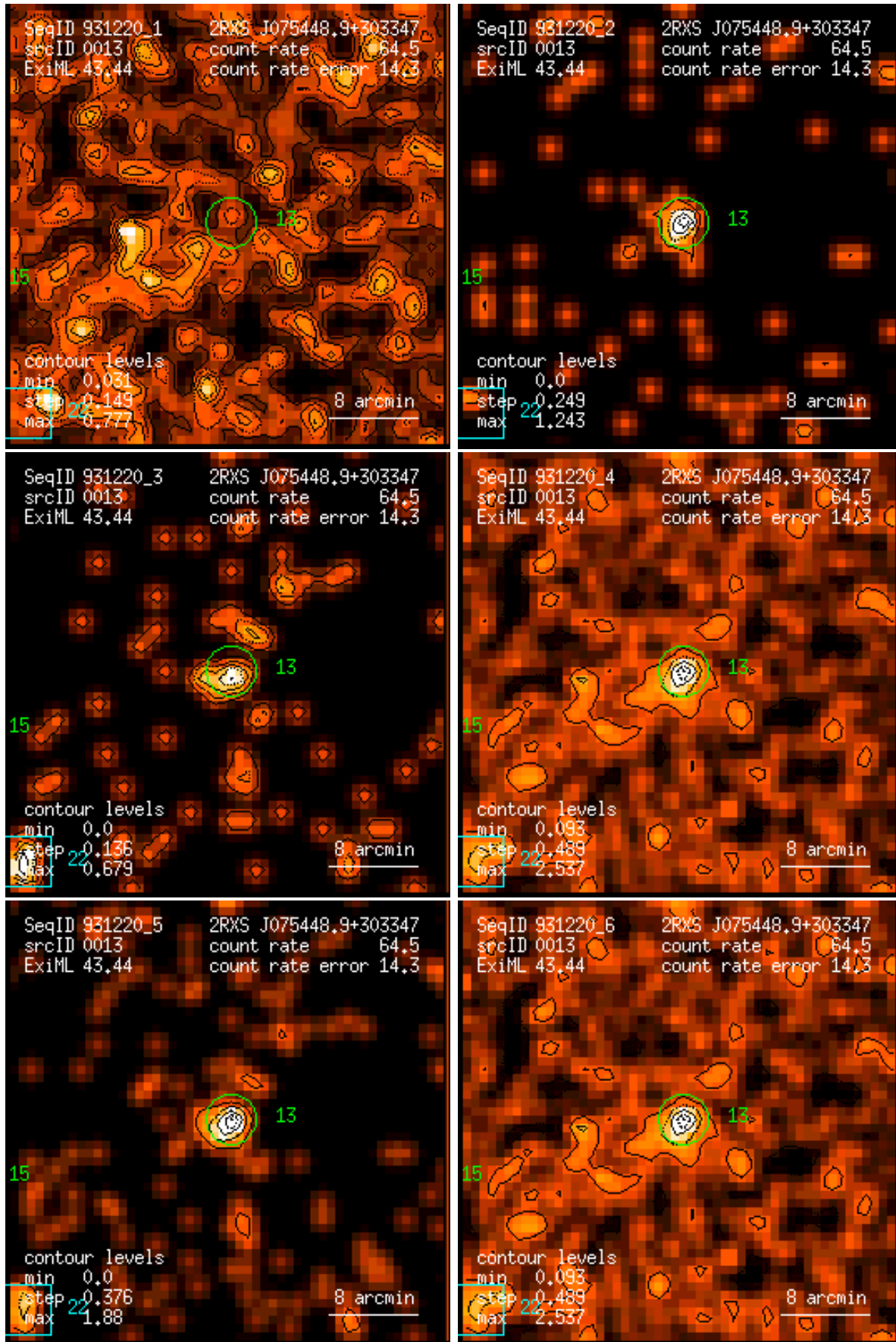
Figure 13: RASS 931220: detection 0013: band rate images, Gaussian filter: (1) PSPC channels 11 – 41, (2) 52 – 90, (3) 91 – 201, (4) 11 – 235, (5) 52 – 201, (6) 11 – 201. Broad band rates in counts/ks. Band rate contour levels in counts/ks/arcmin 2 .
