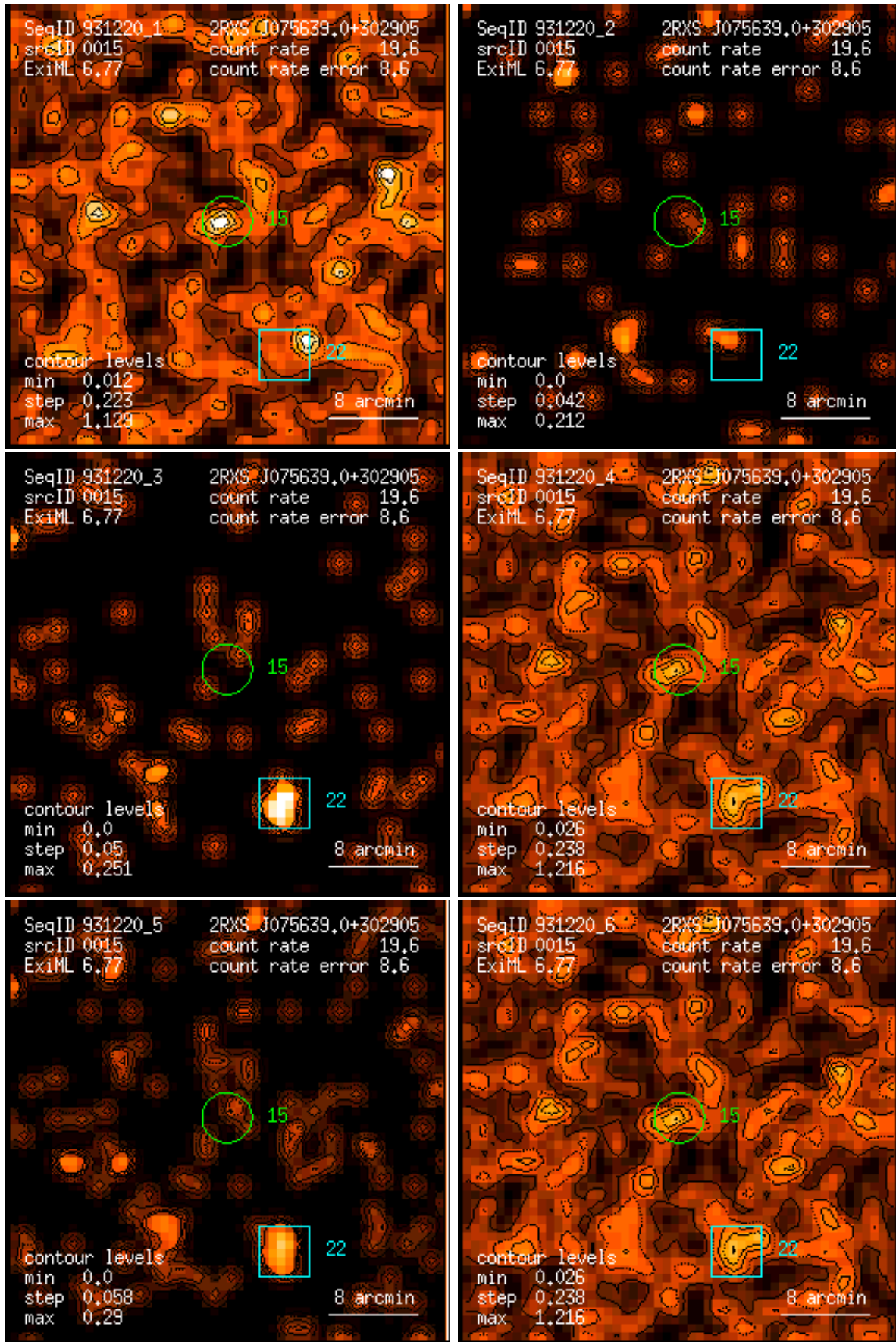
Figure 15: RASS 931220: detection 0015: band rate images, Gaussian filter: (1) PSPC channels 11 – 41, (2) 52 – 90, (3) 91 – 201, (4) 11 – 235, (5) 52 – 201, (6) 11 – 201. Broad band rates in counts/ks. Band rate contour levels in counts/ks/arcmin 2 .
