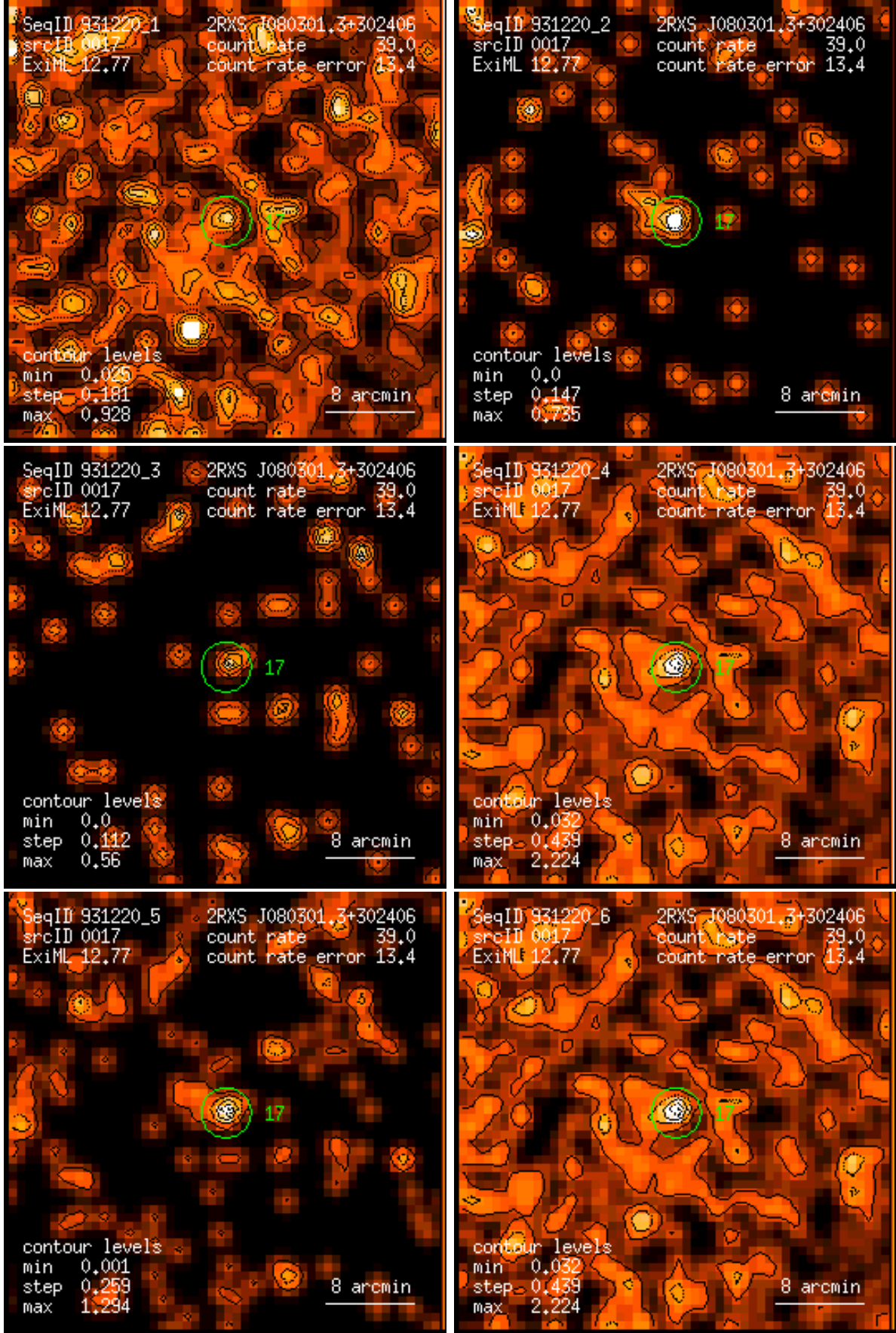
Figure 17: RASS 931220: detection 0017: band rate images, Gaussian filter: (1) PSPC channels 11 – 41, (2) 52 – 90, (3) 91 – 201, (4) 11 – 235, (5) 52 – 201, (6) 11 – 201. Broad band rates in counts/ks. Band rate contour levels in counts/ks/arcmin 2 .
