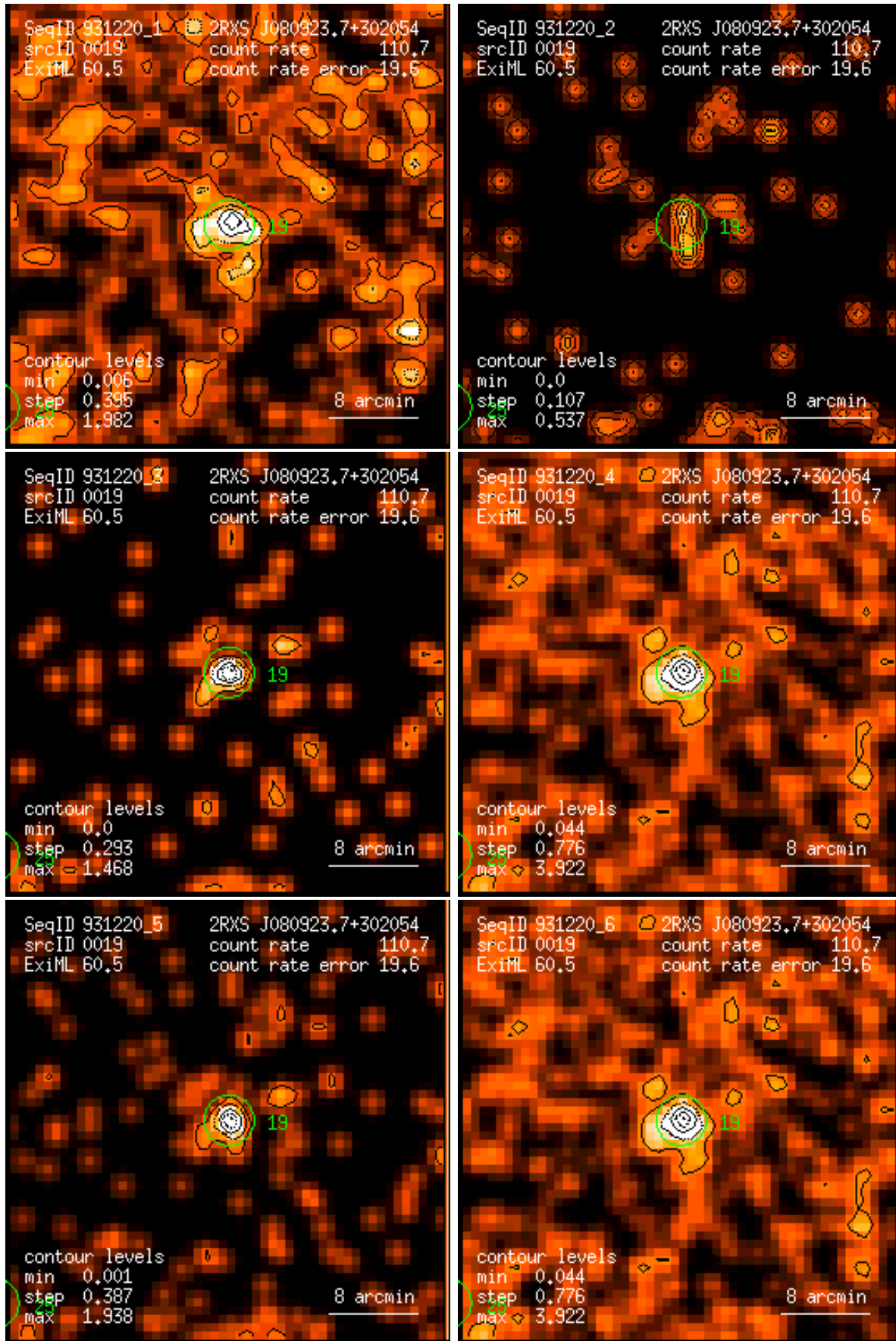
Figure 19: RASS 931220: detection 0019: band rate images, Gaussian filter: (1) PSPC channels 11 – 41, (2) 52 – 90, (3) 91 – 201, (4) 11 – 235, (5) 52 – 201, (6) 11 – 201. Broad band rates in counts/ks. Band rate contour levels in counts/ks/arcmin 2 .
