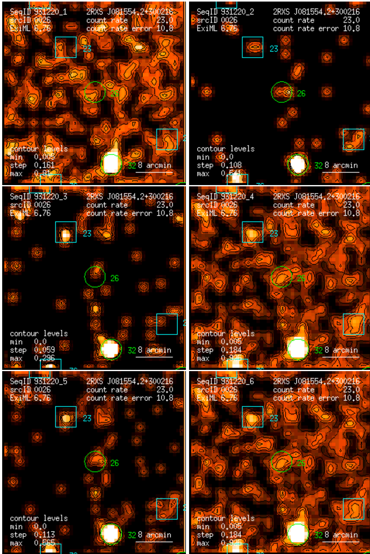
Figure 26: RASS 931220: detection 0026: band rate images, Gaussian filter: (1) PSPC channels 11 – 41, (2) 52 – 90, (3) 91 – 201, (4) 11 – 235, (5) 52 – 201, (6) 11 – 201. Broad band rates in counts/ks. Band rate contour levels in counts/ks/arcmin 2 .
