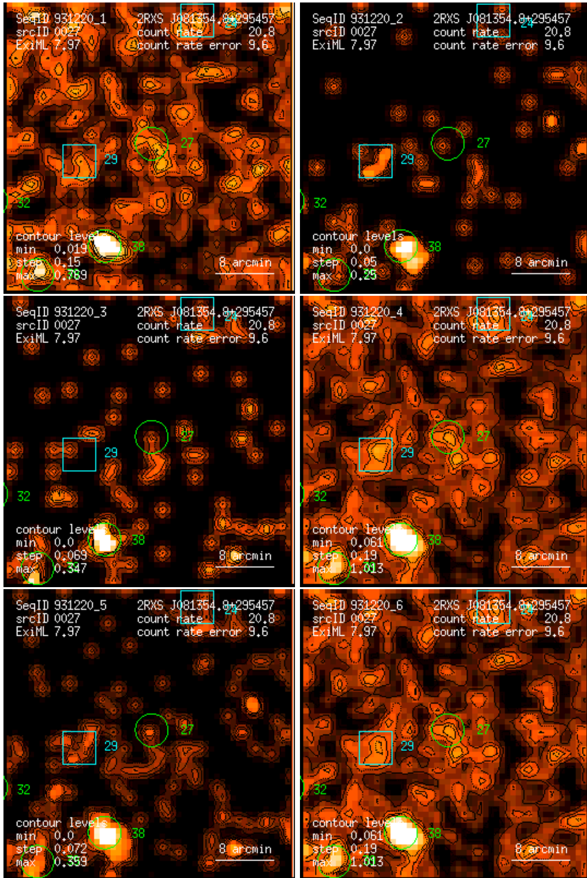
Figure 27: RASS 931220: detection 0027: band rate images, Gaussian filter: (1) PSPC channels 11 – 41, (2) 52 – 90, (3) 91 – 201, (4) 11 – 235, (5) 52 – 201, (6) 11 – 201. Broad band rates in counts/ks. Band rate contour levels in counts/ks/arcmin 2 .
