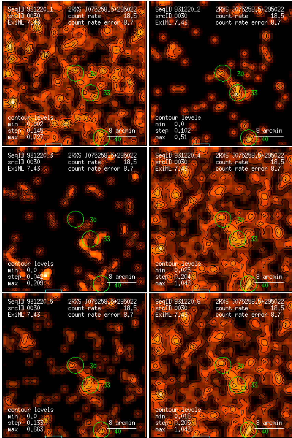
Figure 30: RASS 931220: detection 0030: band rate images, Gaussian filter: (1) PSPC channels 11 – 41, (2) 52 – 90, (3) 91 – 201, (4) 11 – 235, (5) 52 – 201, (6) 11 – 201. Broad band rates in counts/ks. Band rate contour levels in counts/ks/arcmin 2 .
