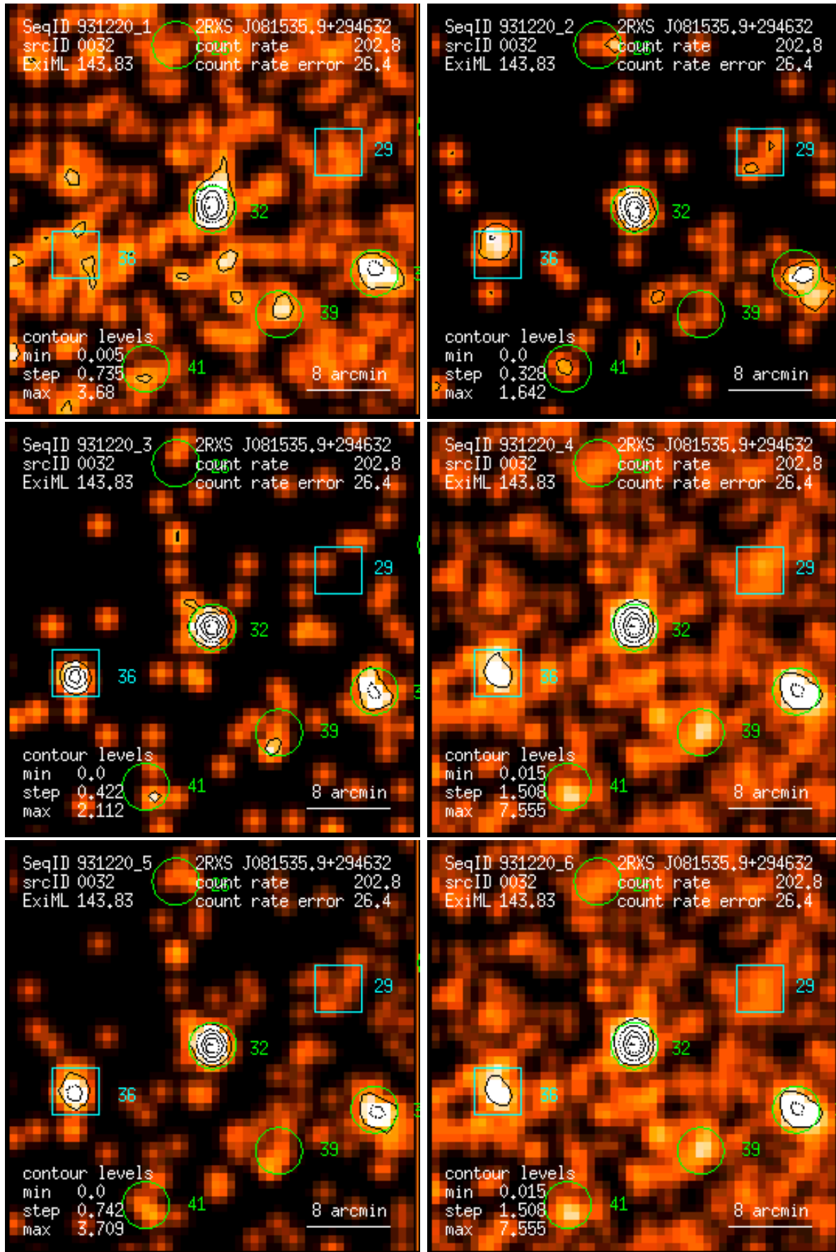
Figure 32: RASS 931220: detection 0032: band rate images, Gaussian filter: (1) PSPC channels 11 – 41, (2) 52 – 90, (3) 91 – 201, (4) 11 – 235, (5) 52 – 201, (6) 11 – 201. Broad band rates in counts/ks. Band rate contour levels in counts/ks/arcmin 2 .
