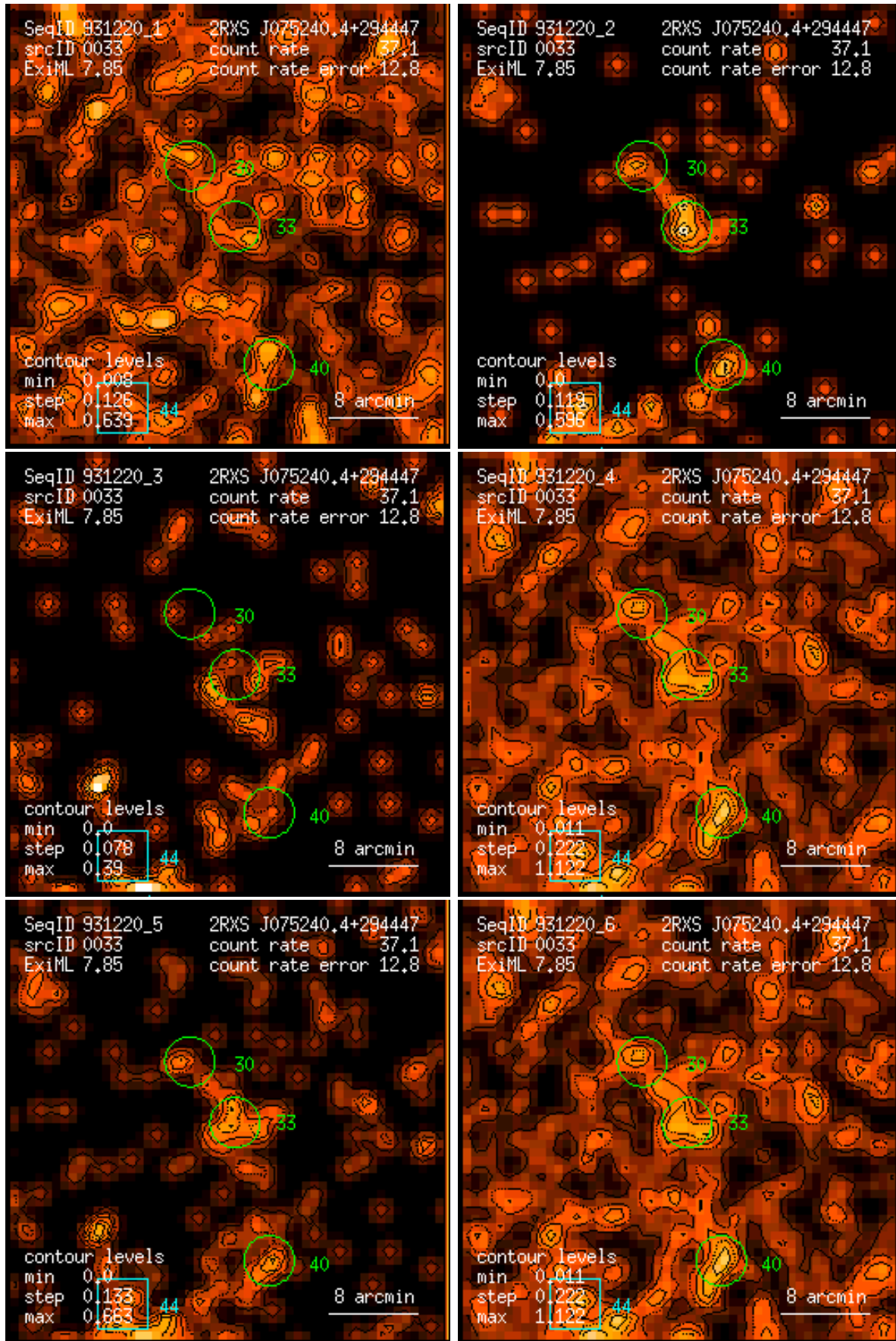
Figure 33: RASS 931220: detection 0033: band rate images, Gaussian filter: (1) PSPC channels 11 – 41, (2) 52 – 90, (3) 91 – 201, (4) 11 – 235, (5) 52 – 201, (6) 11 – 201. Broad band rates in counts/ks. Band rate contour levels in counts/ks/arcmin 2 .
