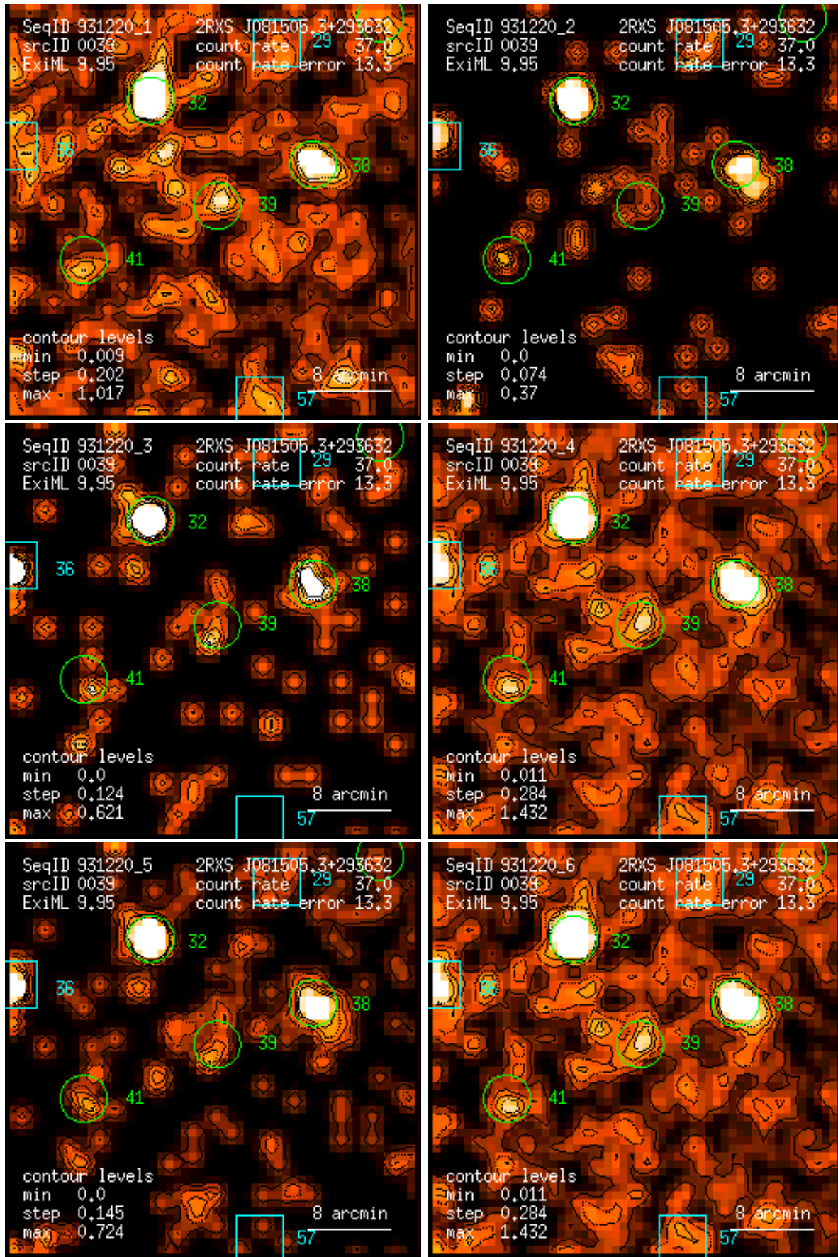
Figure 39: RASS 931220: detection 0039: band rate images, Gaussian filter: (1) PSPC channels 11 – 41, (2) 52 – 90, (3) 91 – 201, (4) 11 – 235, (5) 52 – 201, (6) 11 – 201. Broad band rates in counts/ks. Band rate contour levels in counts/ks/arcmin 2 .
