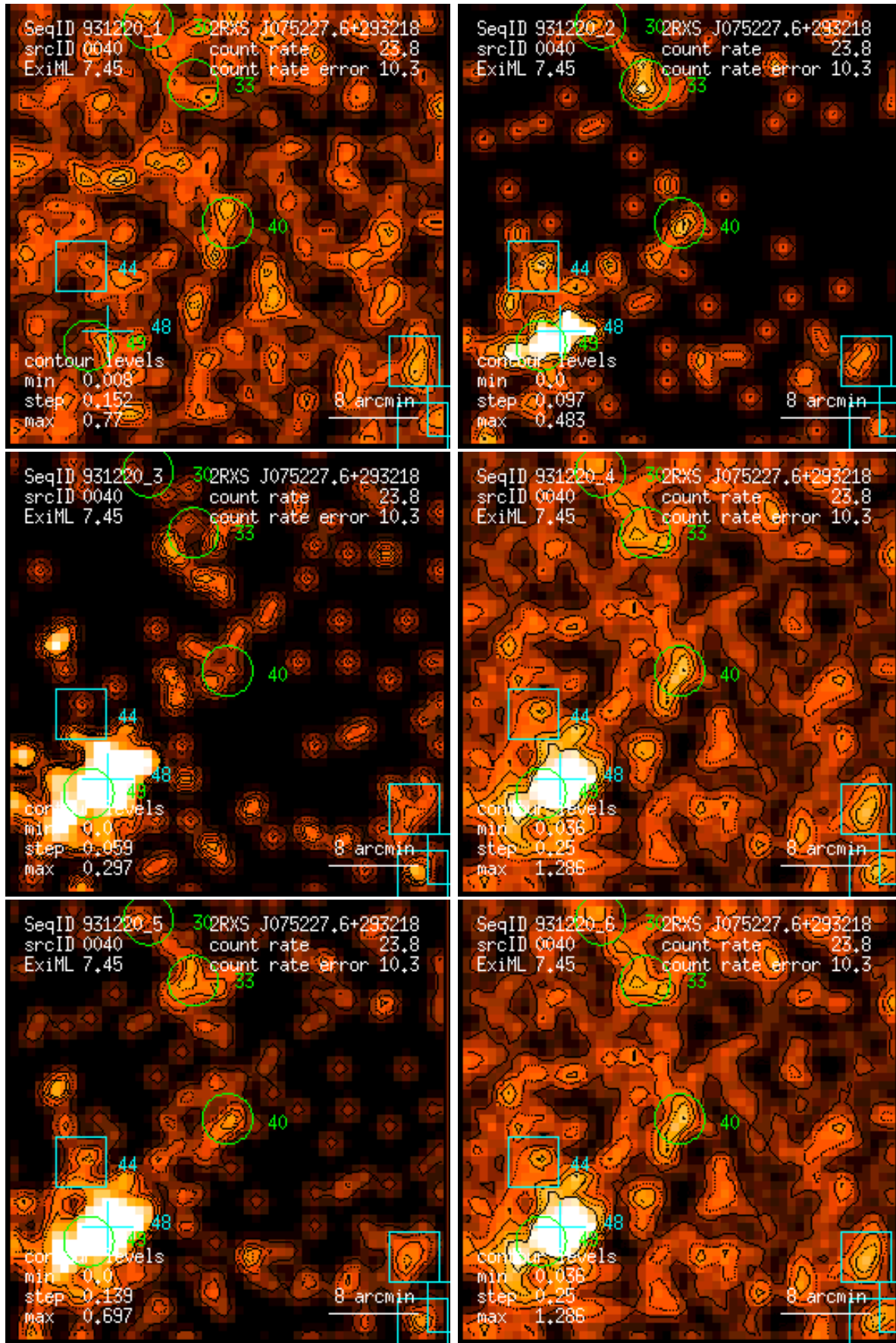
Figure 40: RASS 931220: detection 0040: band rate images, Gaussian filter: (1) PSPC channels 11 – 41, (2) 52 – 90, (3) 91 – 201, (4) 11 – 235, (5) 52 – 201, (6) 11 – 201. Broad band rates in counts/ks. Band rate contour levels in counts/ks/arcmin 2 .
