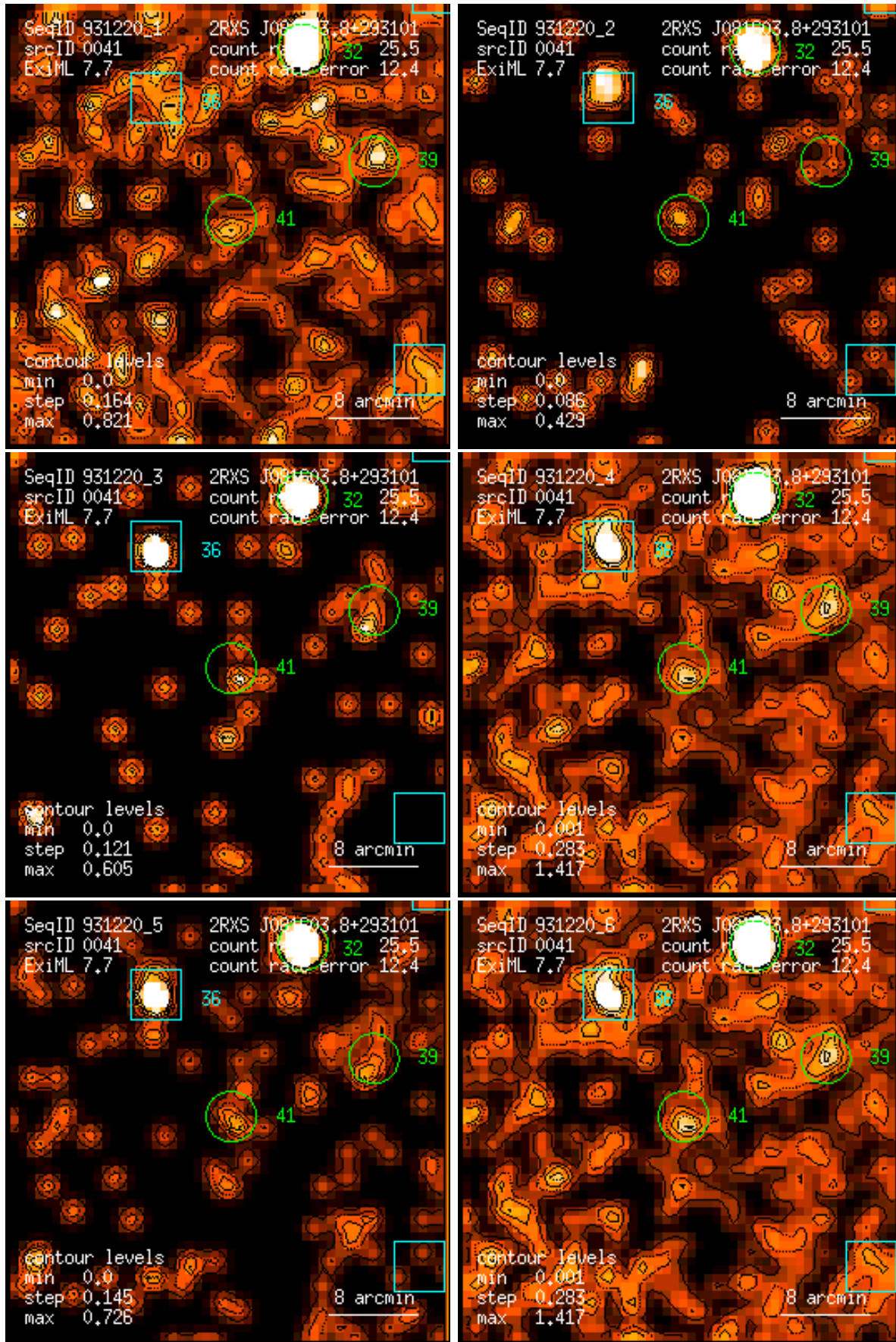
Figure 41: RASS 931220: detection 0041: band rate images, Gaussian filter: (1) PSPC channels 11 – 41, (2) 52 – 90, (3) 91 – 201, (4) 11 – 235, (5) 52 – 201, (6) 11 – 201. Broad band rates in counts/ks. Band rate contour levels in counts/ks/arcmin 2 .
