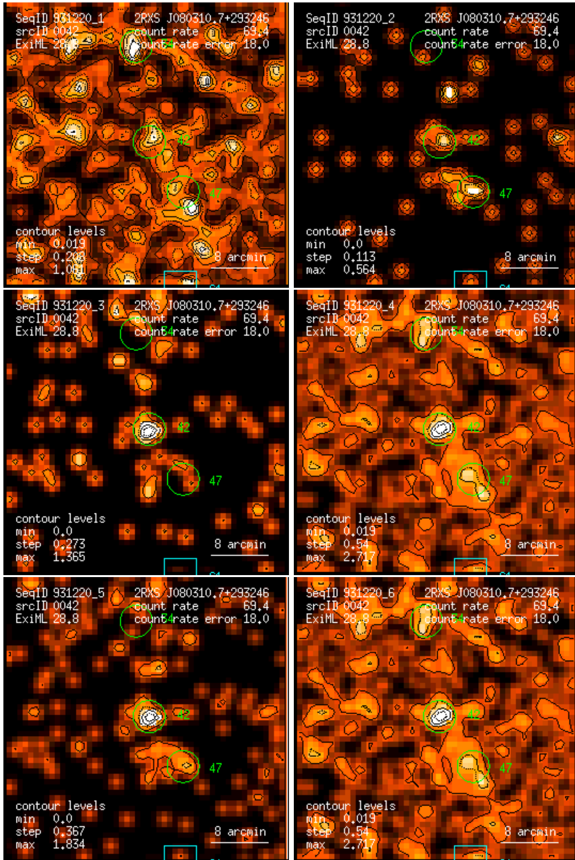
Figure 42: RASS 931220: detection 0042: band rate images, Gaussian filter: (1) PSPC channels 11 – 41, (2) 52 – 90, (3) 91 – 201, (4) 11 – 235, (5) 52 – 201, (6) 11 – 201. Broad band rates in counts/ks. Band rate contour levels in counts/ks/arcmin 2 .
