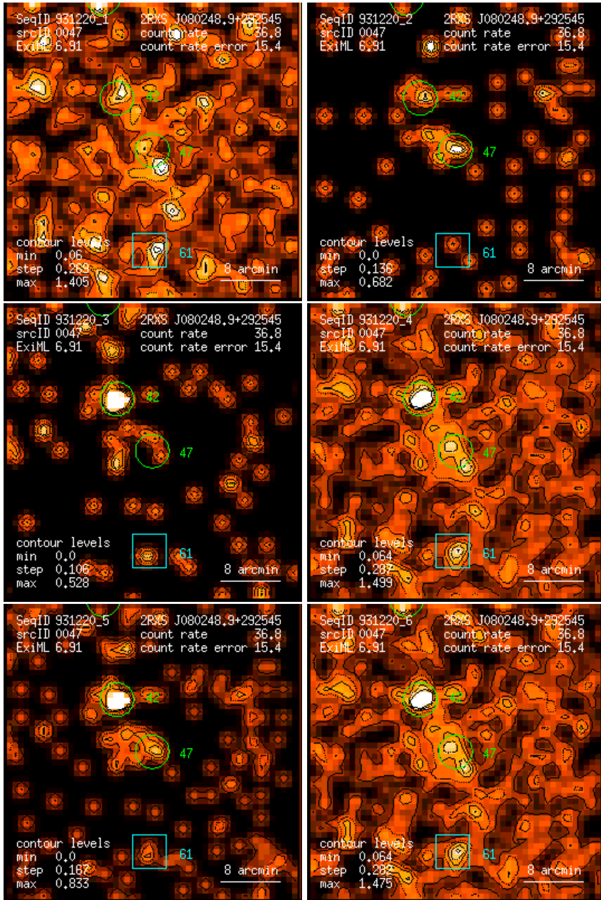
Figure 47: RASS 931220: detection 0047: band rate images, Gaussian filter: (1) PSPC channels 11 – 41, (2) 52 – 90, (3) 91 – 201, (4) 11 – 235, (5) 52 – 201, (6) 11 – 201. Broad band rates in counts/ks. Band rate contour levels in counts/ks/arcmin 2 .
