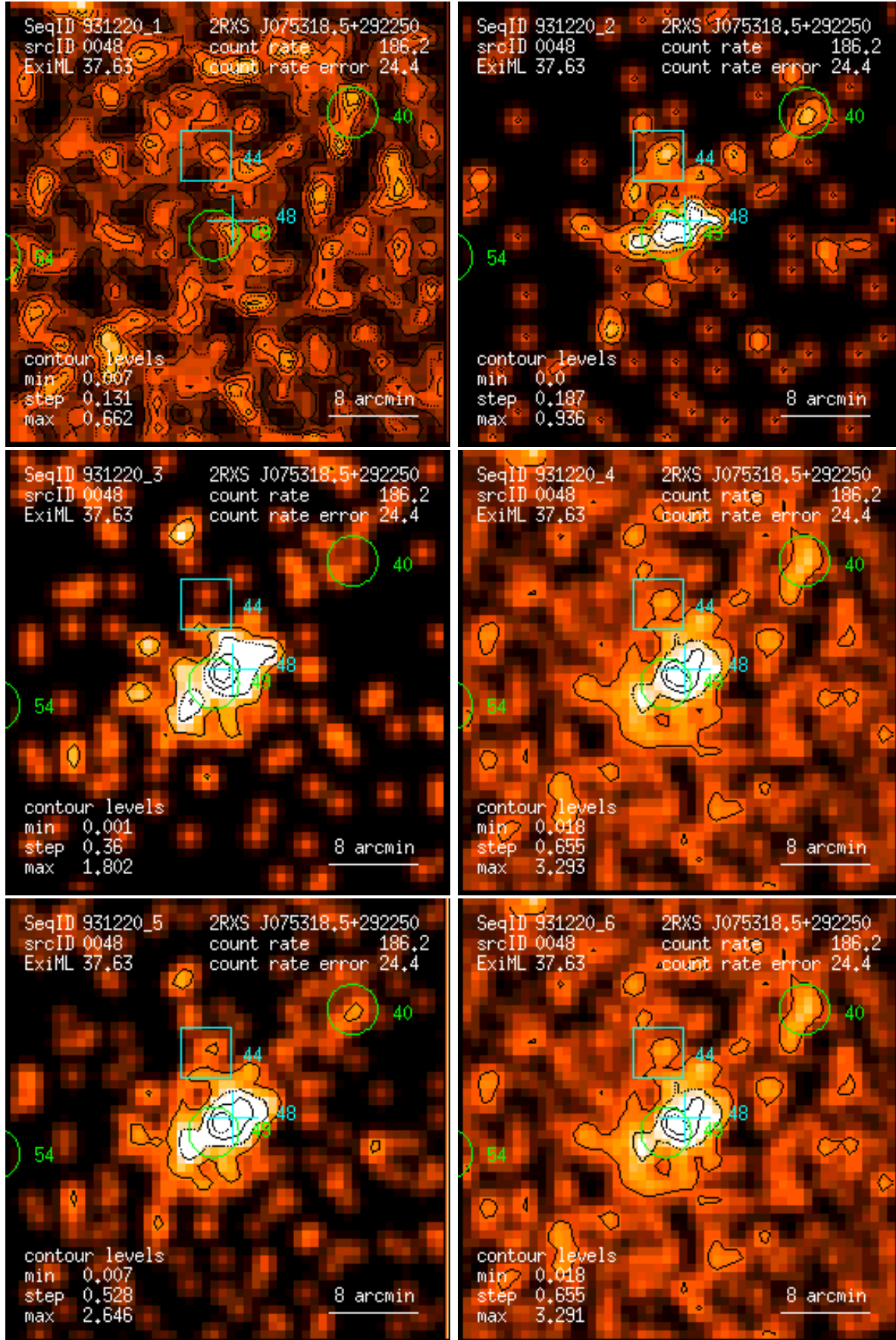
Figure 48: RASS 931220: detection 0048: band rate images, Gaussian filter: (1) PSPC channels 11 – 41, (2) 52 – 90, (3) 91 – 201, (4) 11 – 235, (5) 52 – 201, (6) 11 – 201. Broad band rates in counts/ks. Band rate contour levels in counts/ks/arcmin 2 .
