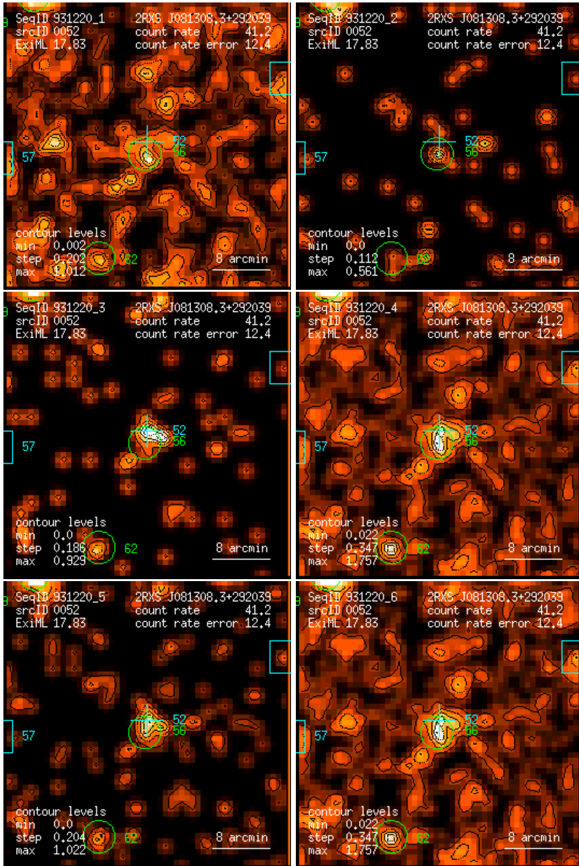
Figure 52: RASS 931220: detection 0052: band rate images, Gaussian filter: (1) PSPC channels 11 – 41, (2) 52 – 90, (3) 91 – 201, (4) 11 – 235, (5) 52 – 201, (6) 11 – 201. Broad band rates in counts/ks. Band rate contour levels in counts/ks/arcmin 2 .
