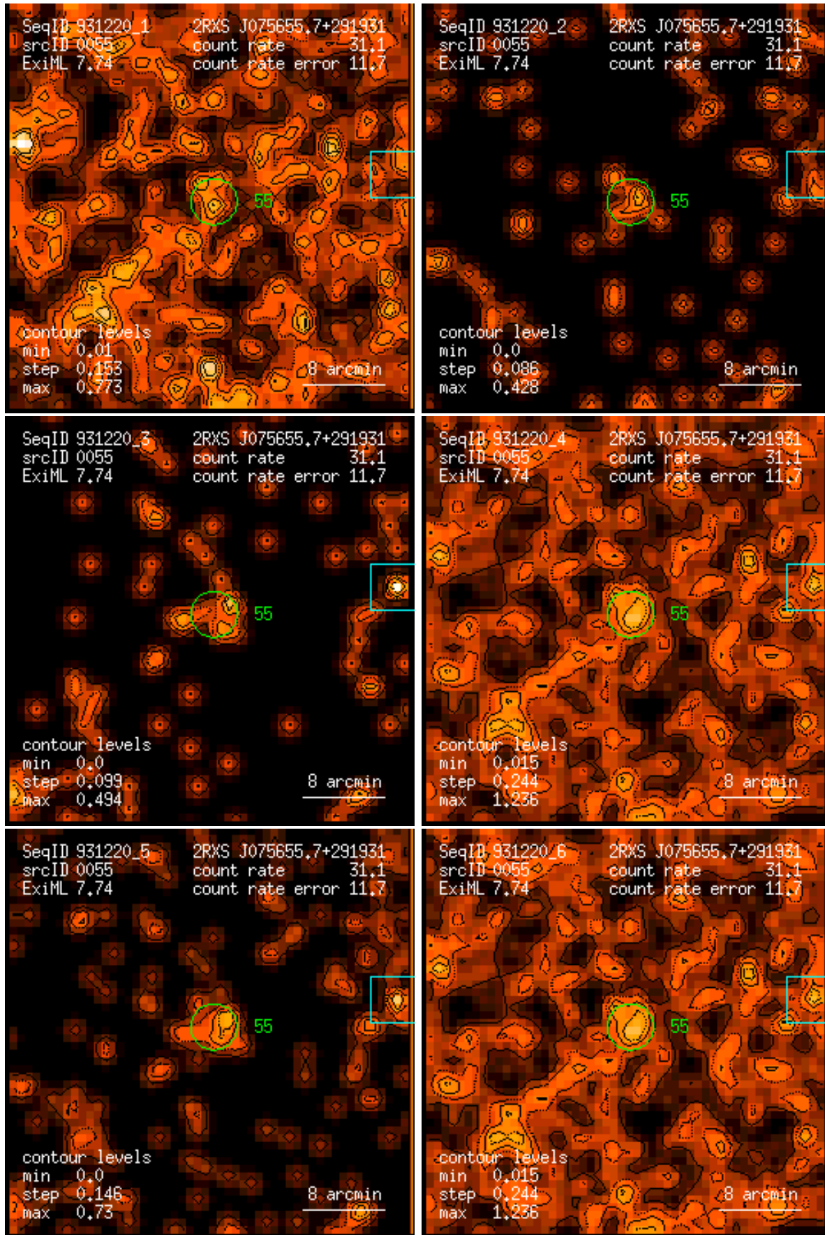
Figure 55: RASS 931220: detection 0055: band rate images, Gaussian filter: (1) PSPC channels 11 – 41, (2) 52 – 90, (3) 91 – 201, (4) 11 – 235, (5) 52 – 201, (6) 11 – 201. Broad band rates in counts/ks. Band rate contour levels in counts/ks/arcmin 2 .
