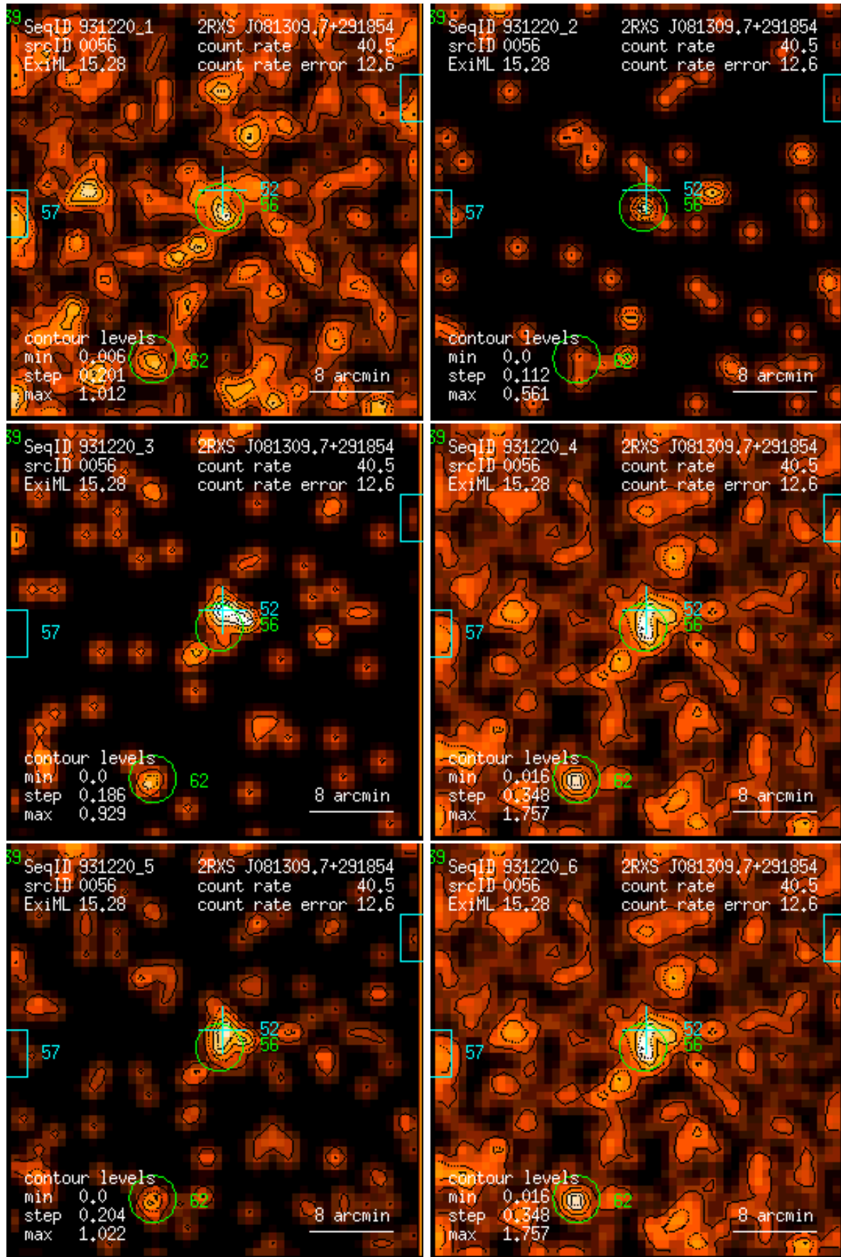
Figure 56: RASS 931220: detection 0056: band rate images, Gaussian filter: (1) PSPC channels 11 – 41, (2) 52 – 90, (3) 91 – 201, (4) 11 – 235, (5) 52 – 201, (6) 11 – 201. Broad band rates in counts/ks. Band rate contour levels in counts/ks/arcmin 2 .
