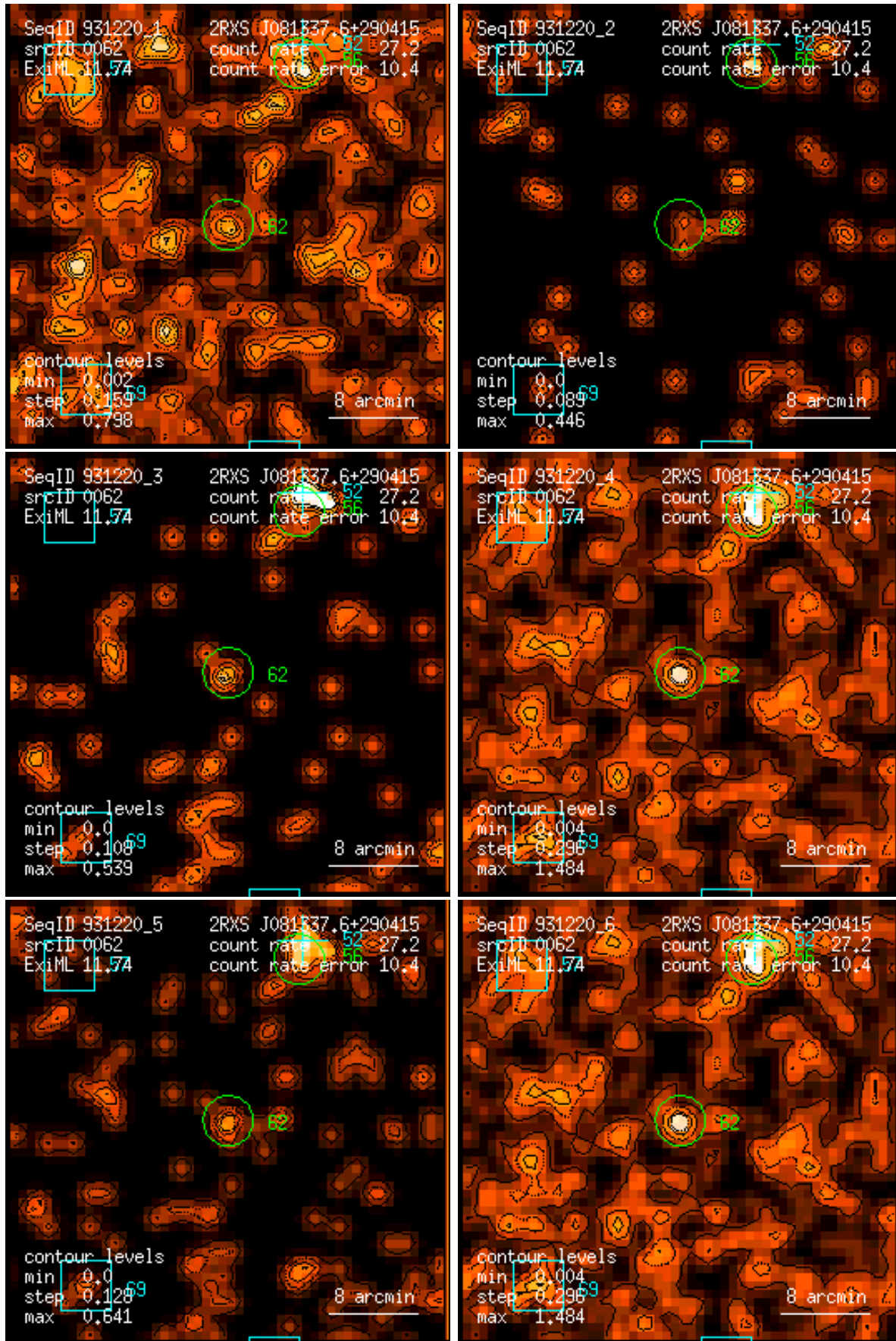
Figure 62: RASS 931220: detection 0062: band rate images, Gaussian filter: (1) PSPC channels 11 – 41, (2) 52 – 90, (3) 91 – 201, (4) 11 – 235, (5) 52 – 201, (6) 11 – 201. Broad band rates in counts/ks. Band rate contour levels in counts/ks/arcmin 2 .
