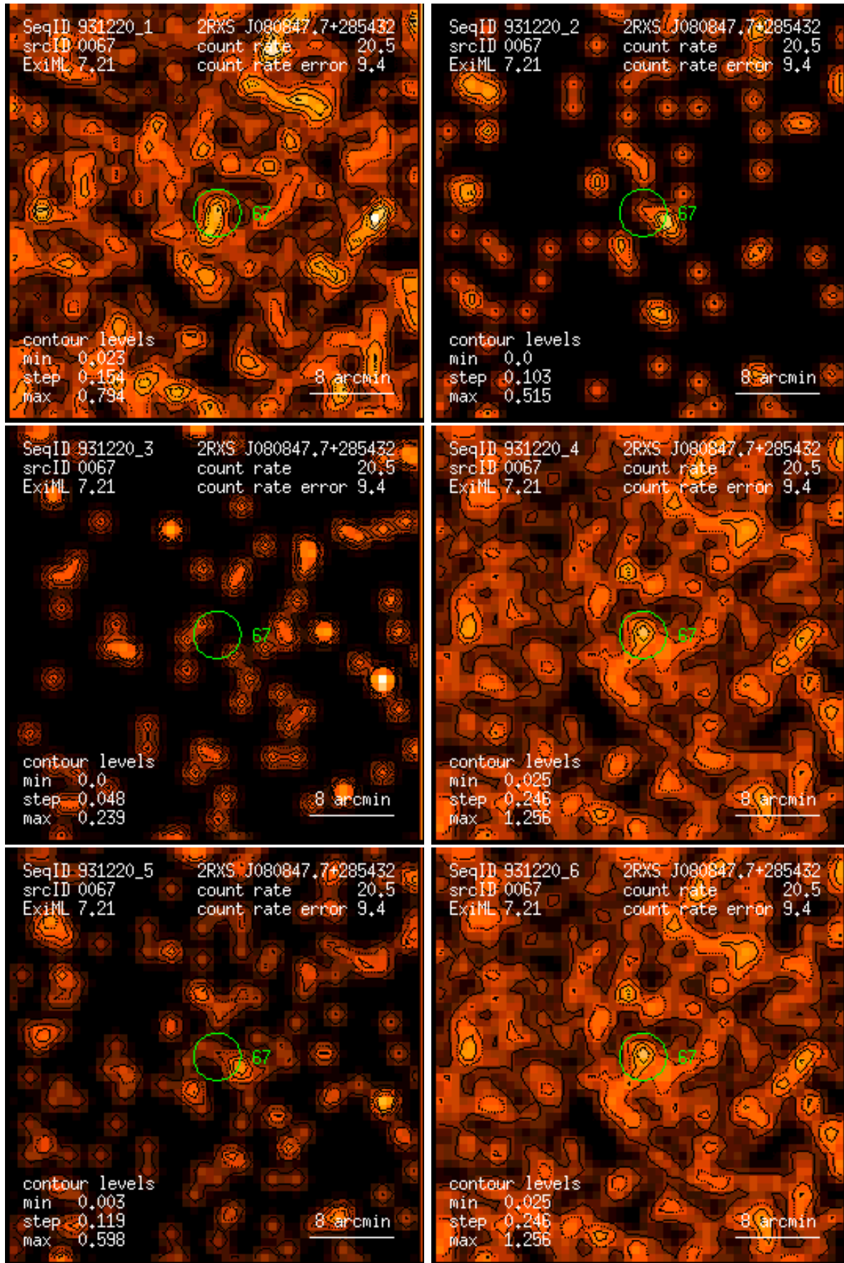
Figure 67: RASS 931220: detection 0067: band rate images, Gaussian filter: (1) PSPC channels 11 – 41, (2) 52 – 90, (3) 91 – 201, (4) 11 – 235, (5) 52 – 201, (6) 11 – 201. Broad band rates in counts/ks. Band rate contour levels in counts/ks/arcmin 2 .
